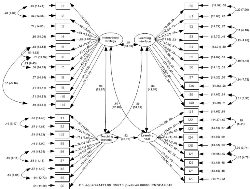
Figure 1. Confirmatory Factor Analysis (CFA) model.
