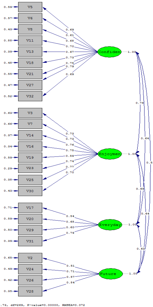
Figure 1. The path diagram for the four-factor model
