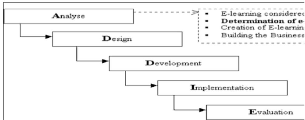
Figure 1: Theoretical Framework
