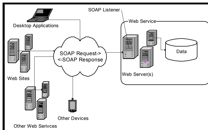
Figure 5: Logical architecture of a web service built on the flexible services architecture
