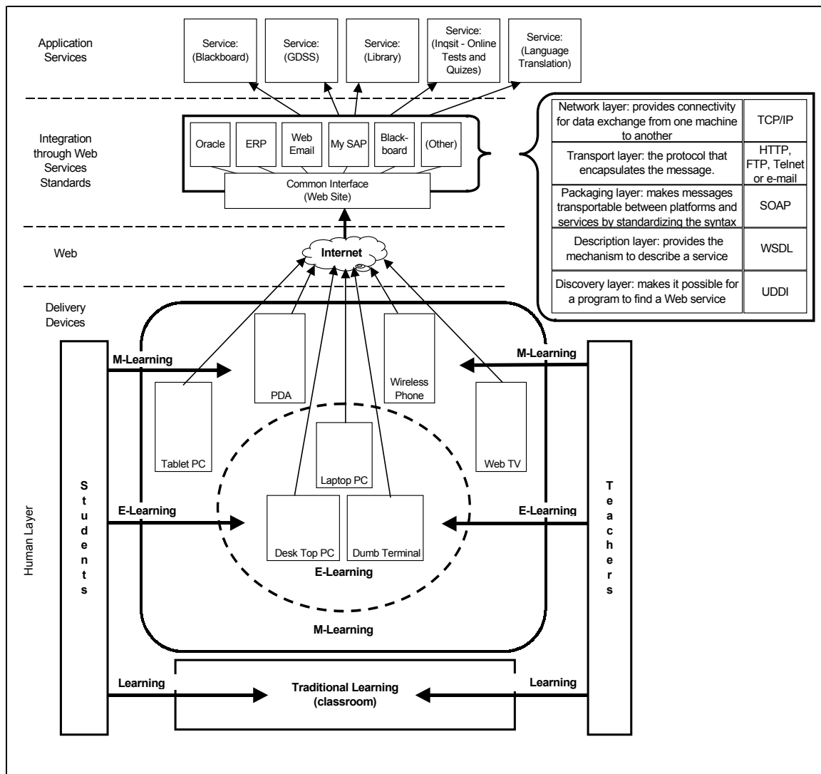
Figure 6: Flexible services architecture for web services
