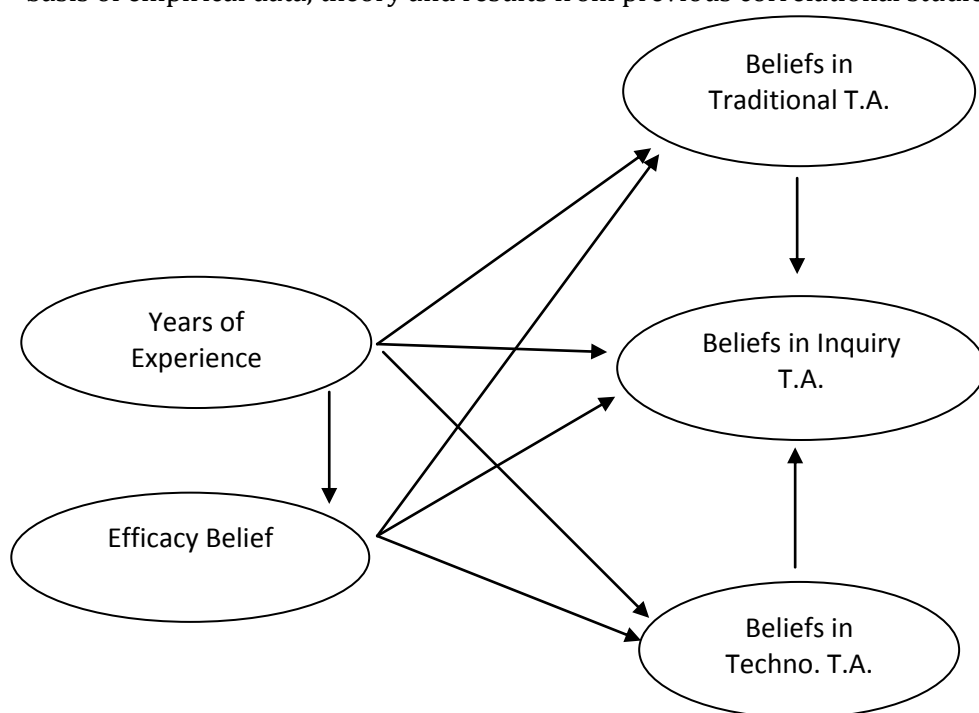
Figure 1. Hypothesized Model
