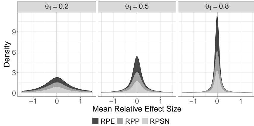
FIG 2. This plot shows the density of the estimated mean relative effect size H when the true mean relative effect size is \eta = 0 . Each panel shows the distribution of H when effects in the replication study are zero (i.e., \theta_{2j} = 0 ) and effects in the original studies are small ( \theta_1 = 0.2 ), medium ( \theta_1 = 0.5 ), or large ( \theta_1 = 0.8 ). Within each panel, the colors correspond to the distribution of H for each replication research program. Note that an accurate estimate would correspond to H \approx 0 , and an inaccurate estimate would correspond to H \approx 1 or -1 .
