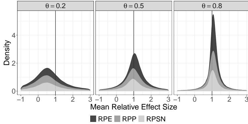
FIG 1. This plot shows the density of the estimated mean relative effect size H when the true mean relative effect size is \eta = 1 . Each panel shows the distribution of H when effects in each pair of studies are the same size and are small ( \theta = 0.2 ), medium ( \theta = 0.5 ), or large ( \theta = 0.8 ). Within each panel, the colors correspond to the distribution of H for each replication research program. Note that an accurate estimate would correspond to H \approx 1
