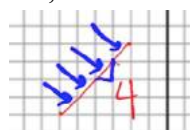
Figure 2 – Line drawn through square diagonals
