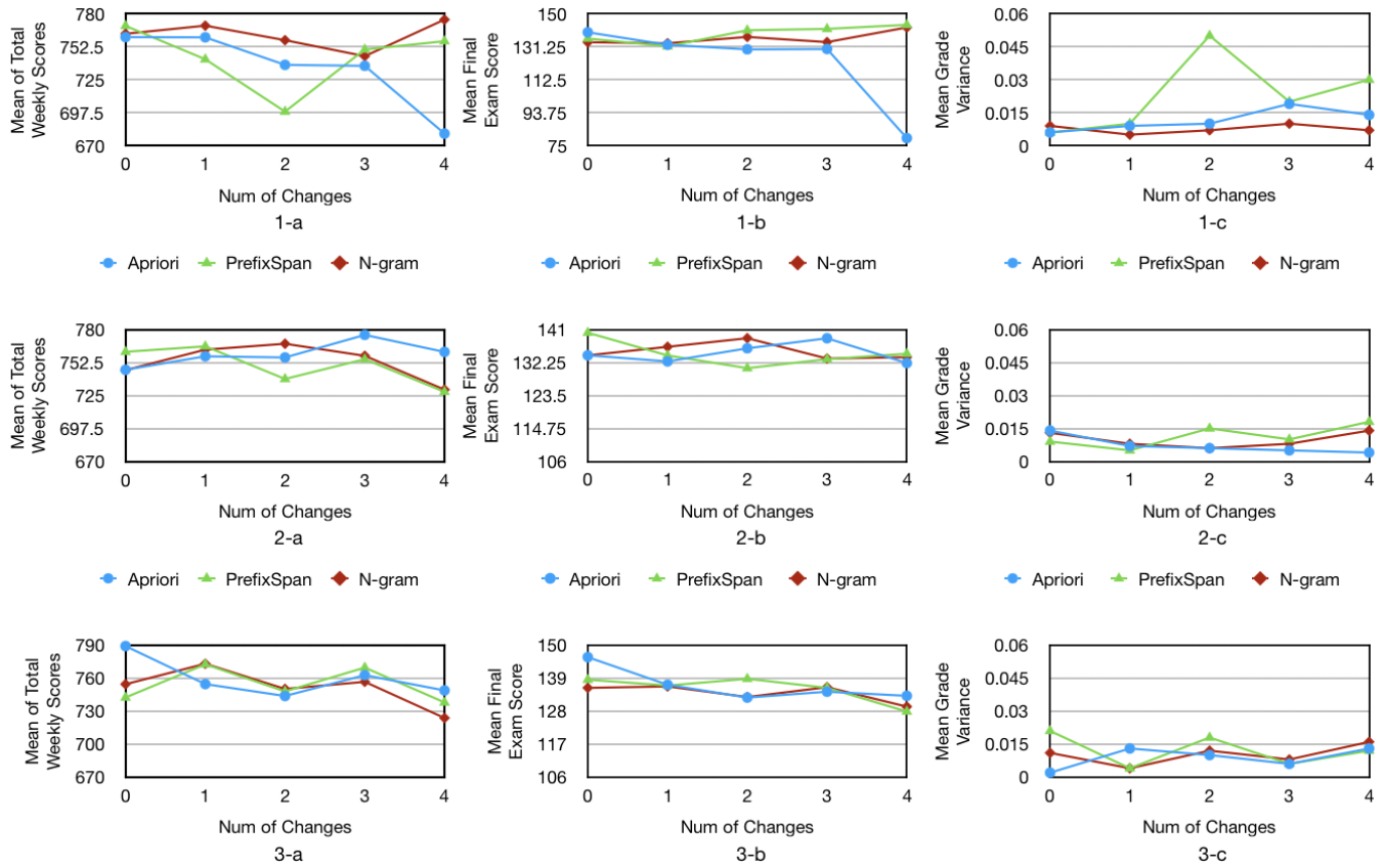
Figure 1: Comparison between different clustering algorithms with different pattern mining algorithms. 1: Spectral Clustering. 2: Agglomerative Clustering. 3: K-means. a. Relationship between number of changes and mean of total weekly scores. b. Relationship between number of changes and mean final exam score. c. Relationship between number of changes and mean grade variance.
