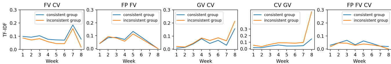
Figure 3: Average TF-IDF values in each week for students in C1
