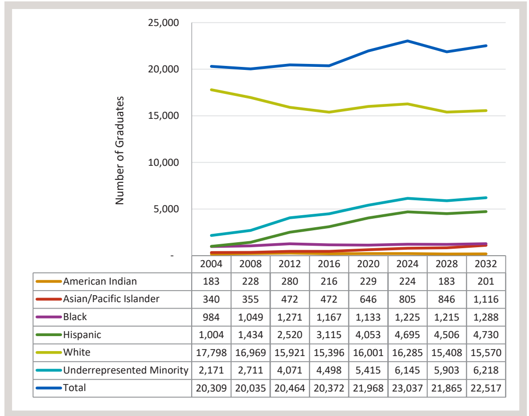
Figure 4. Public High School Graduate Trends in Nebraska Through 2032 by Race and Ethnicity
