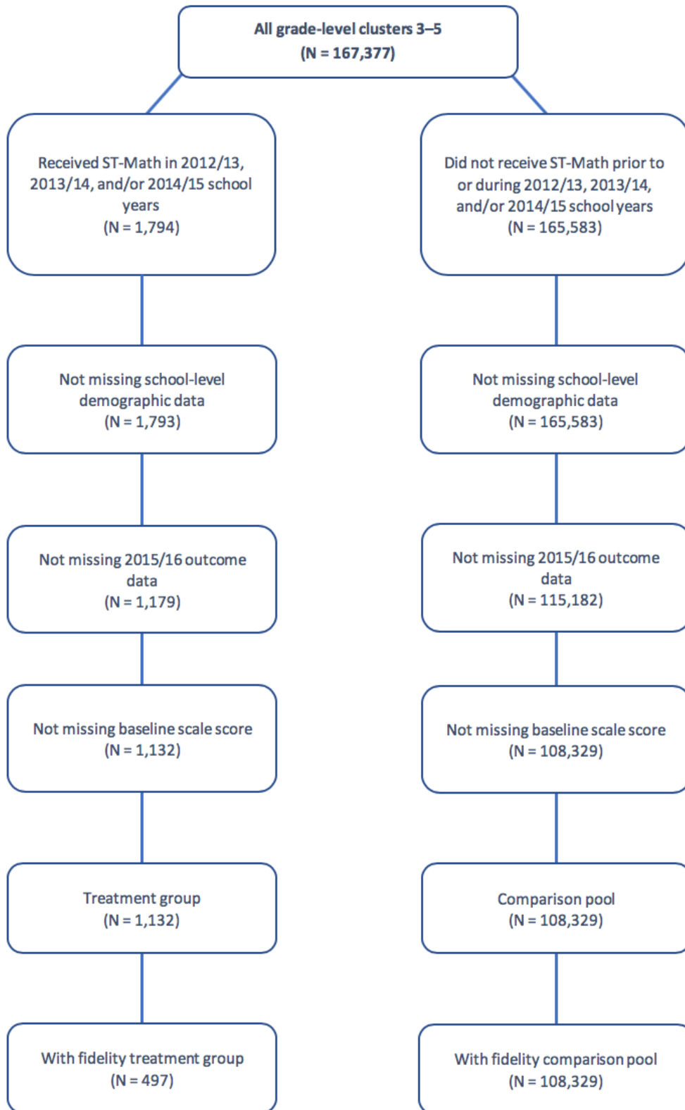
Exhibit C1. Consort Diagram
