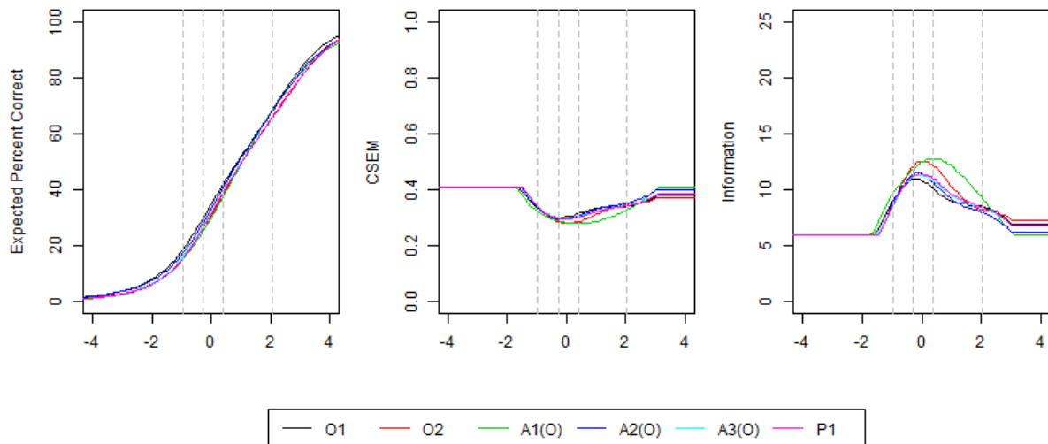
Figure 12.1 Test Characteristic Curves, Conditional Standard Error of Measurement Curves, and Information Curves for ELA/L Grade 3
