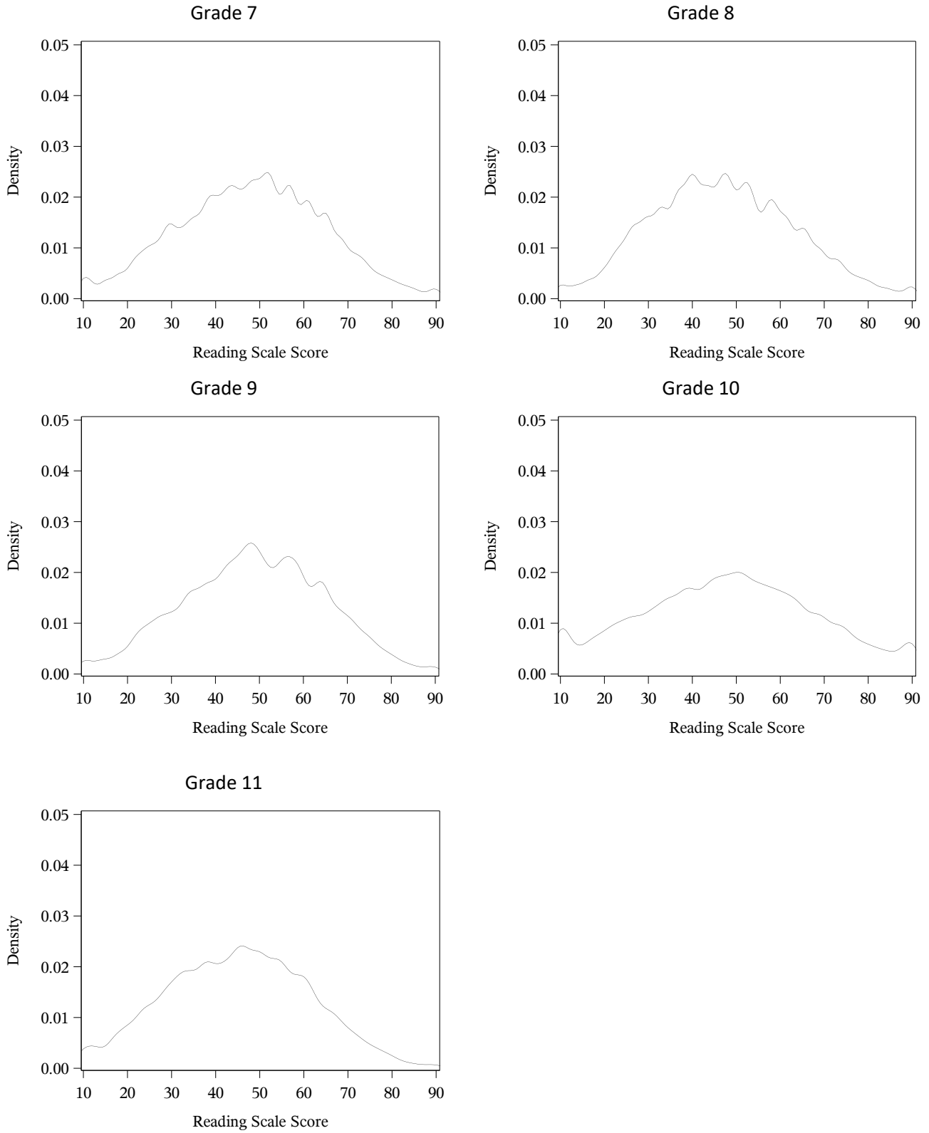
Figure 12.3 (continued) Distributions of Reading Scale Scores: Grades 3–11
