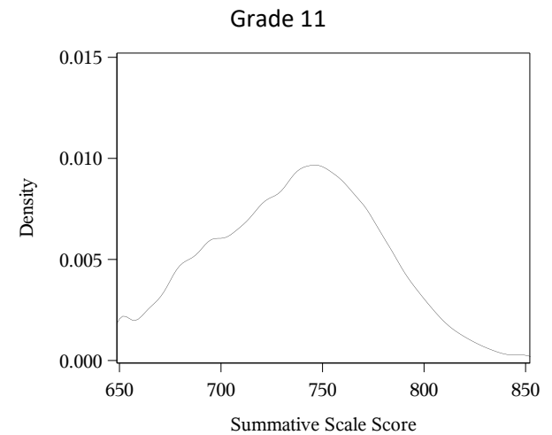
Figure 12.2 (continued) Distributions of ELA/L Scale Scores: Grades 3–11
