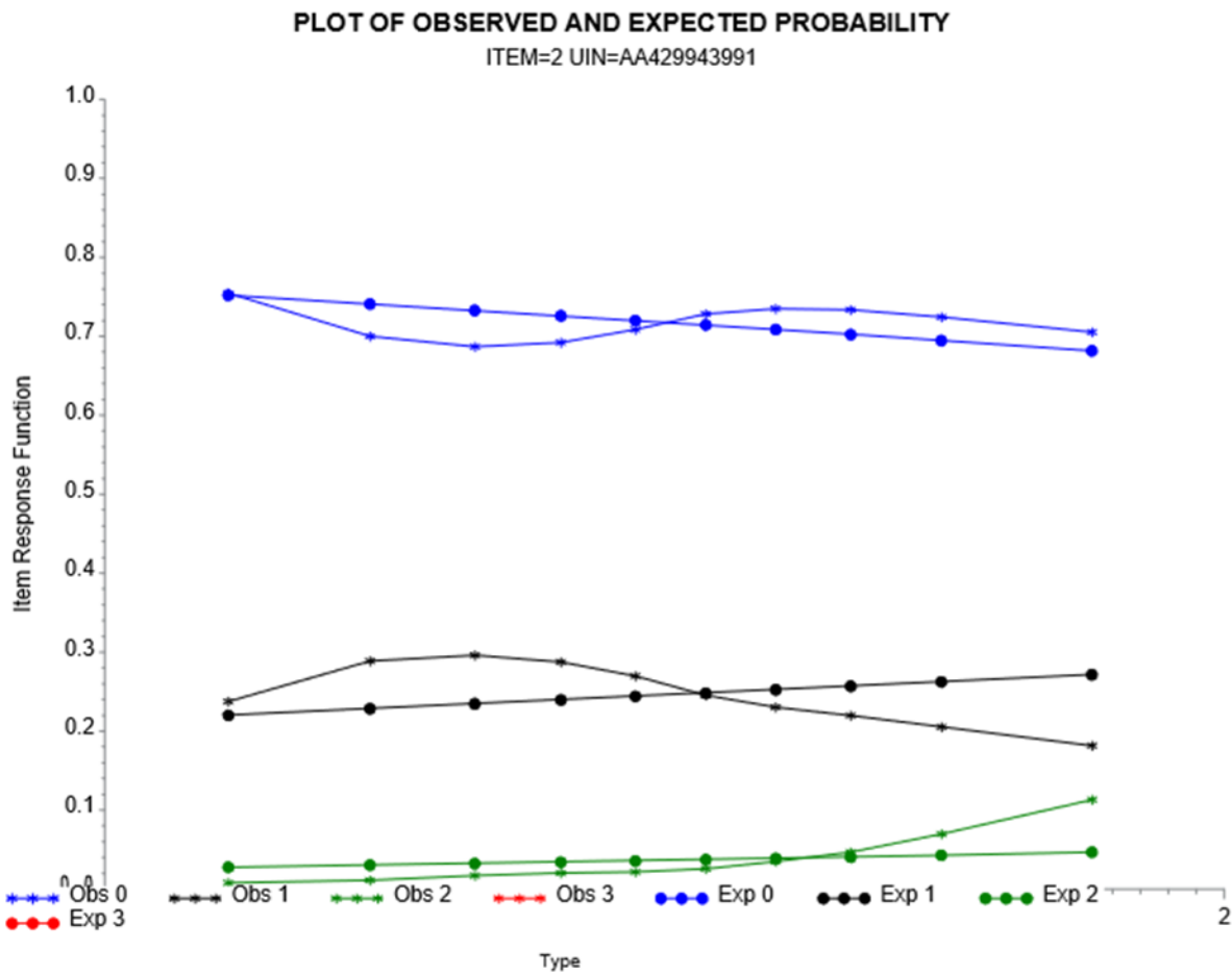
Figure 10.2 An example ELA/L 3-Category Item, 2 PL/GPC Model, n-count 100,622
