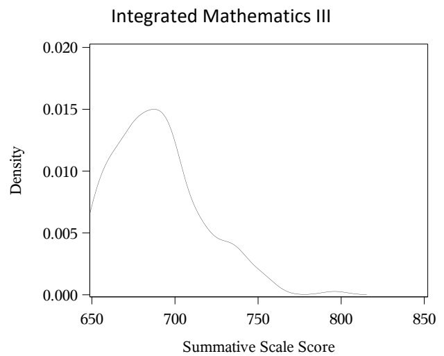
Figure 12.6 Distributions of Mathematics Scale Scores: High School
