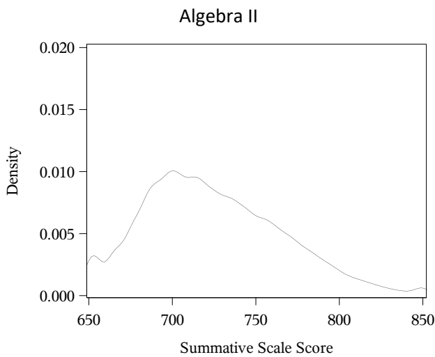
Figure 12.6 Distributions of Mathematics Scale Scores: High School
