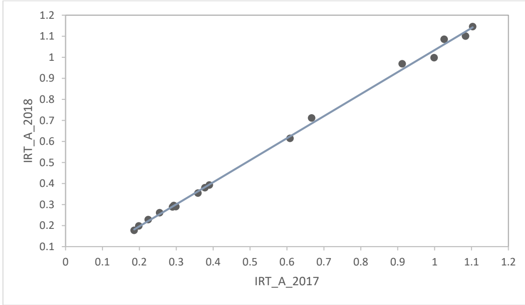
Figure 10.3 ELA/L Grade 8 Transformed New a - vs. Reference a -Parameter Estimates for Year-to-Year Linking
