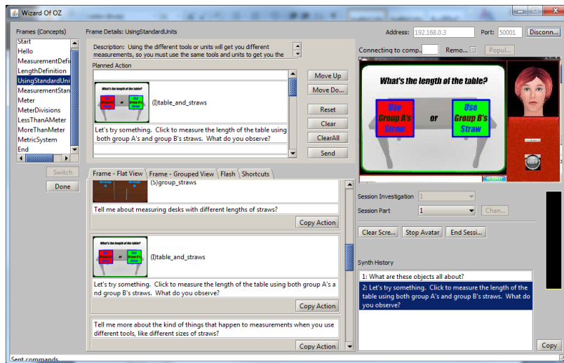
Figure 6 - Wizard screen
