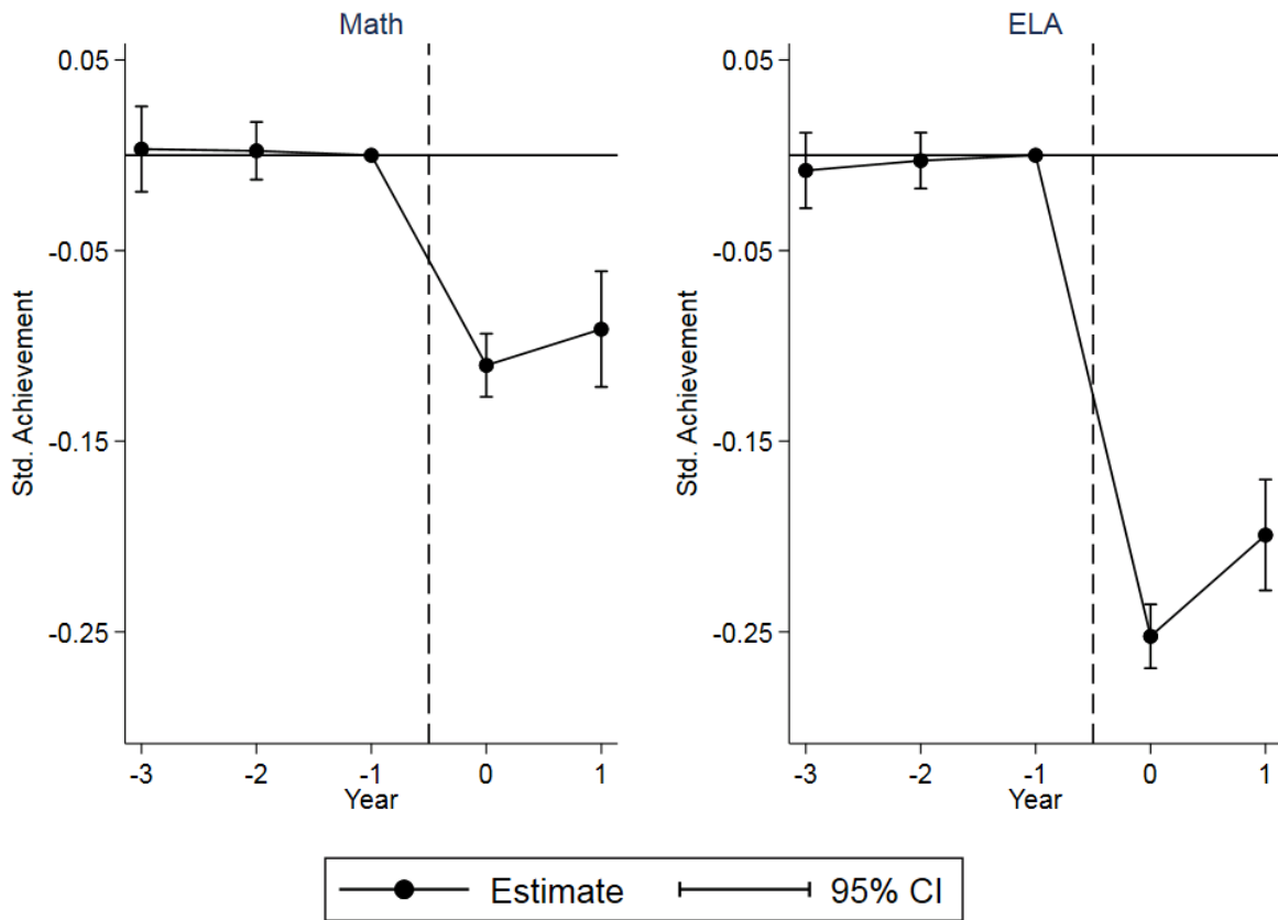
Figure 5. Effects of computer-based testing by year relative to implementation
