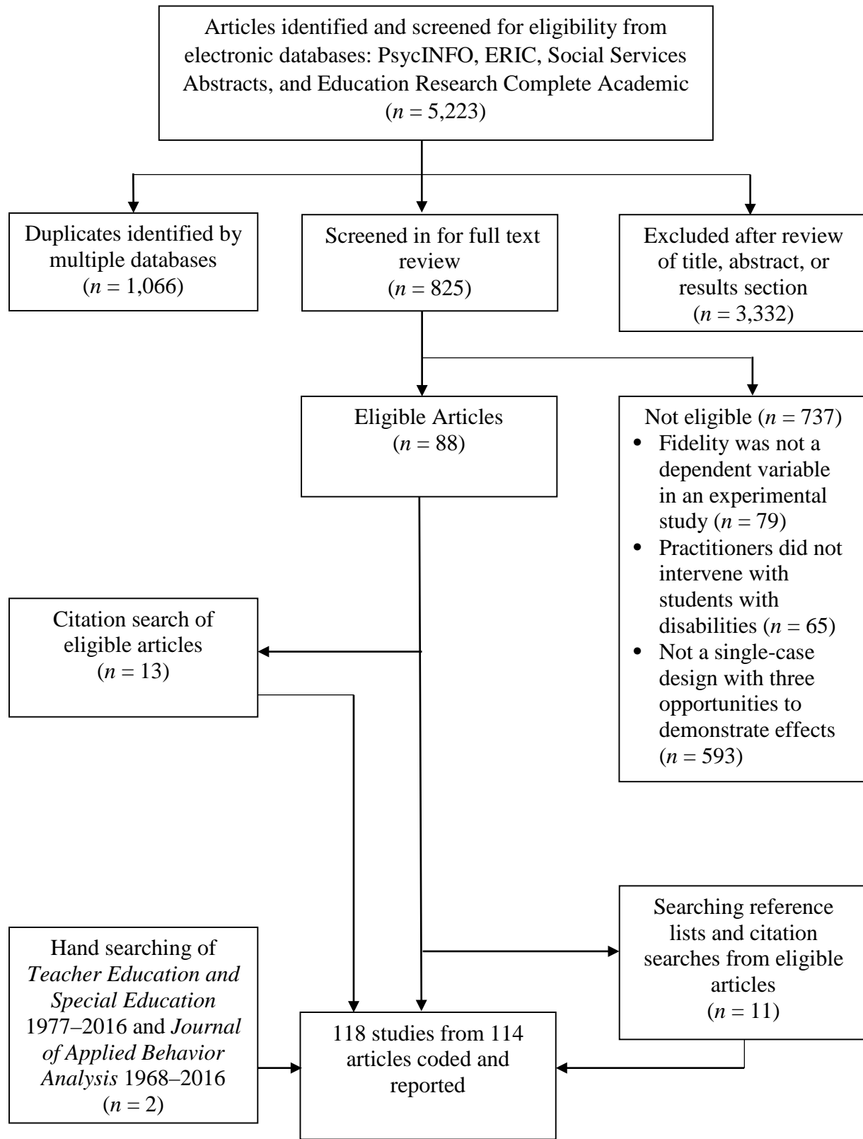
Figure 1. Flow diagram of study search procedures.
