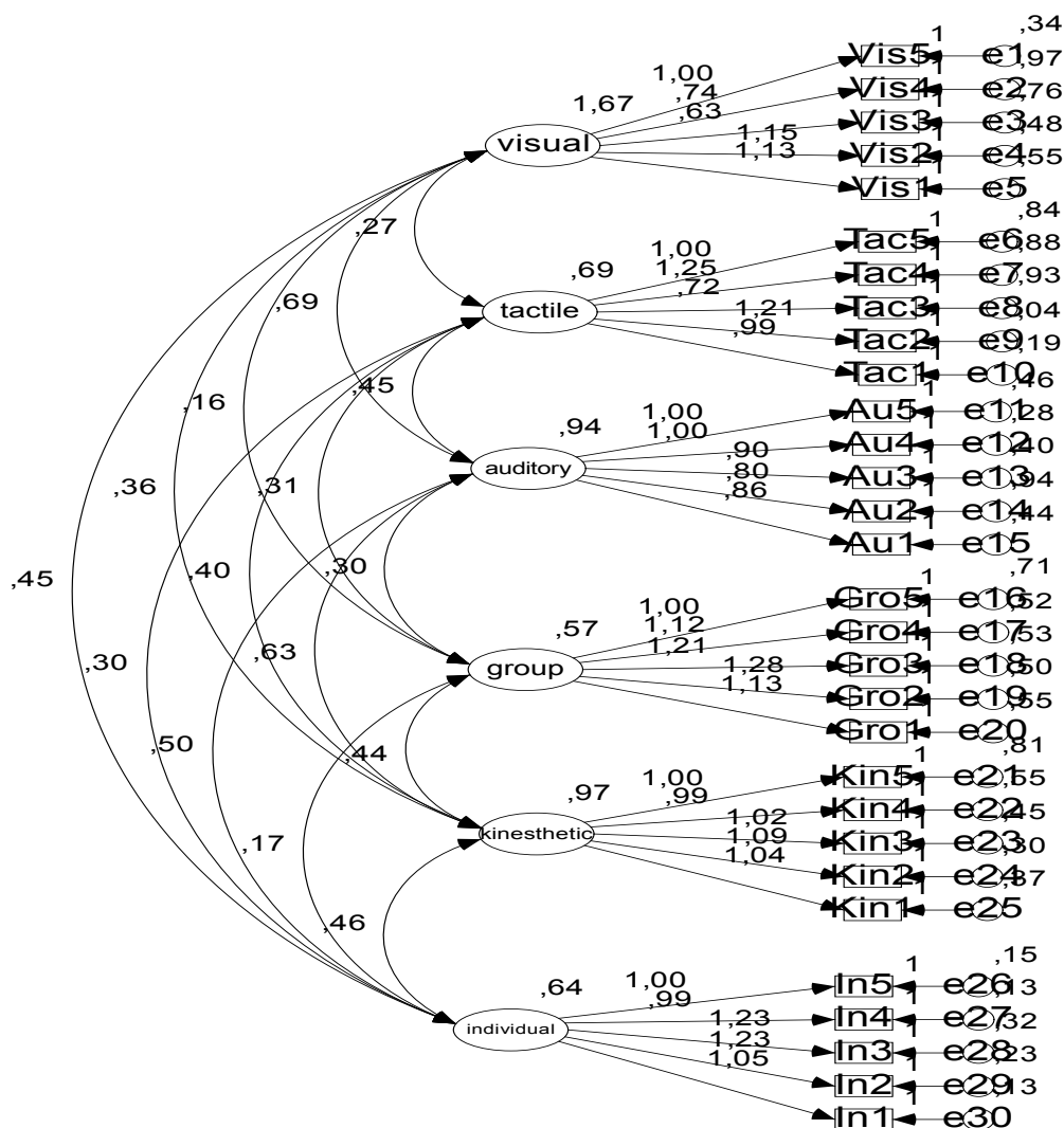
Graph 4.1. CFA results
