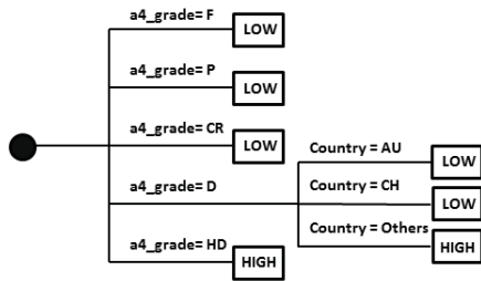
Figure 2. Tree Produced by the Standard DT
