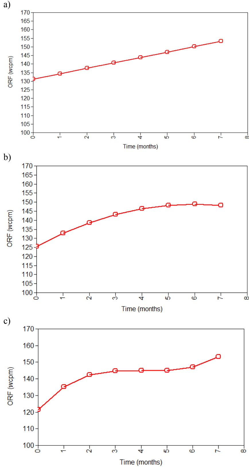
Figure 2. (a) Predicted (estimated) linear mean ORF growth across time. (b) Predicted quadratic mean ORF growth across time. (c) Predicted cubic mean ORF growth across time.
