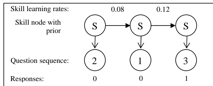
Figure 2. Bayesian network model for question sequence [2 1 3]
