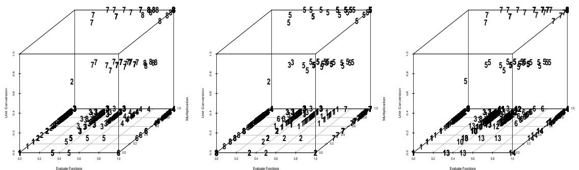
Figure 1: Cluster Assignments: a) HC, Complete G=8 ; b) K-means G=8 ; c) MBC G=14
