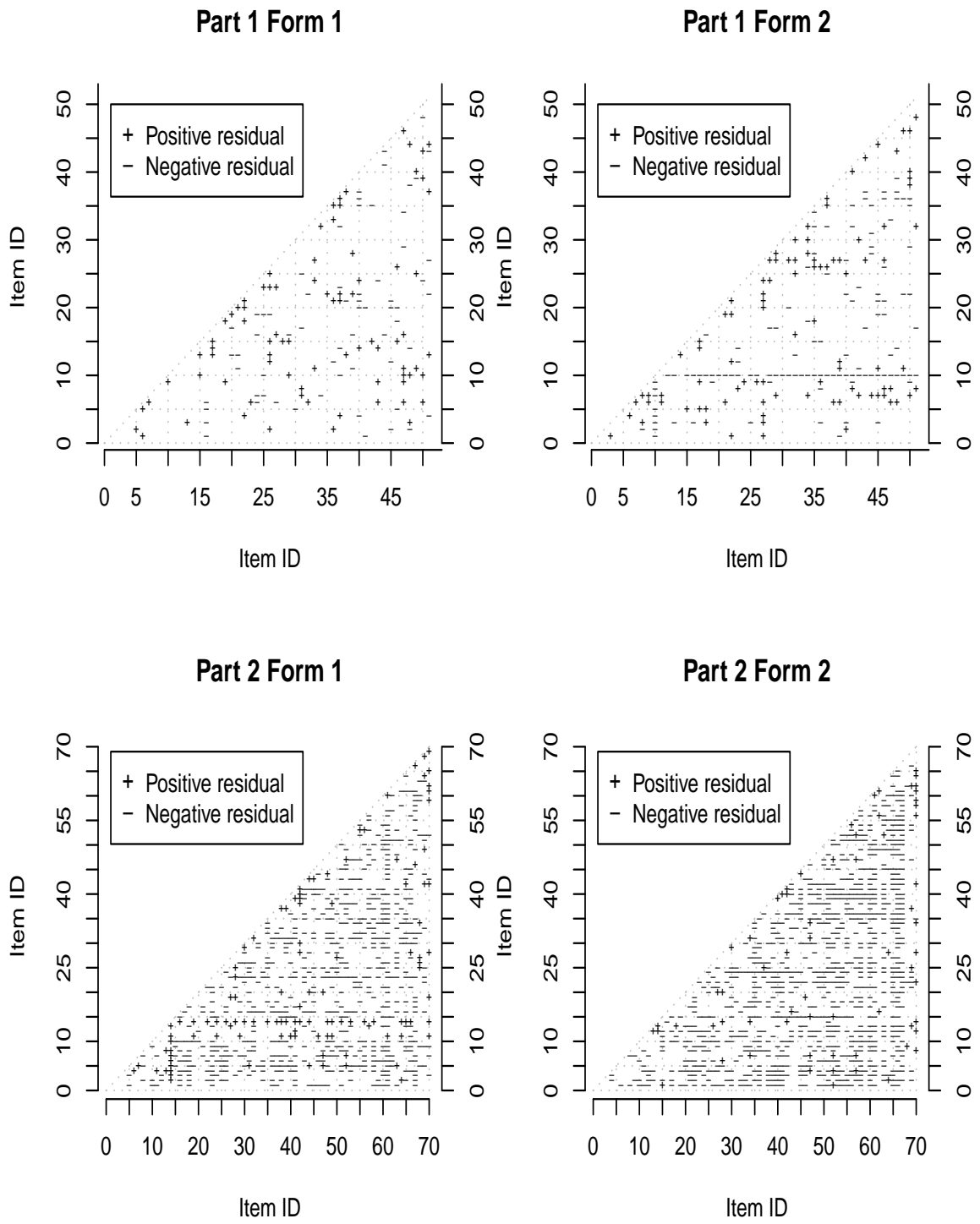
Figure 23. The fit of the IRT model to the second-order marginal totals for the English proficiency test.
