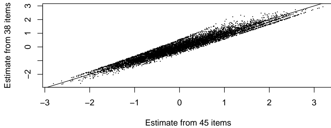
Scatter-plot of the Two Sets of Ability Estimates
