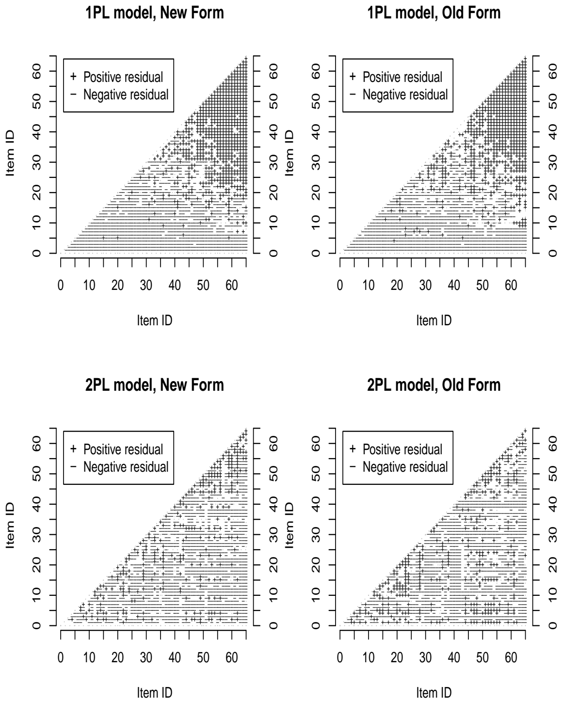
Figure 39. The fit of the IRT model to the second-order marginal totals for the state test: Subject 1.
