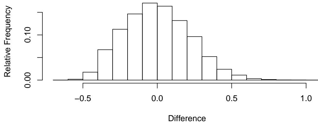
Histogram of Differences in Ability Estimates
