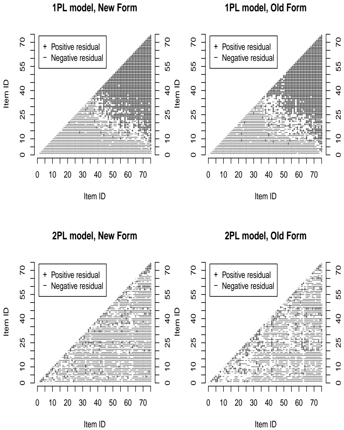
Figure 41. The fit of the IRT model to the second-order marginal totals for the state test: Subject 3.
