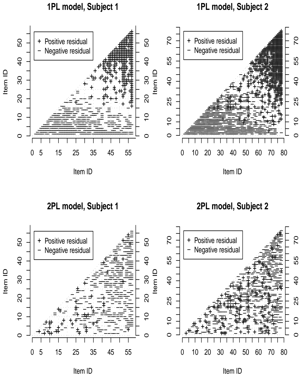
Figure 31. The fit of the IRT model to the second-order marginal totals for the battery of examinations.
