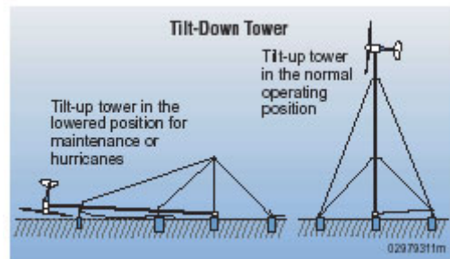
Figure 42 – Tilt-Down Towers
