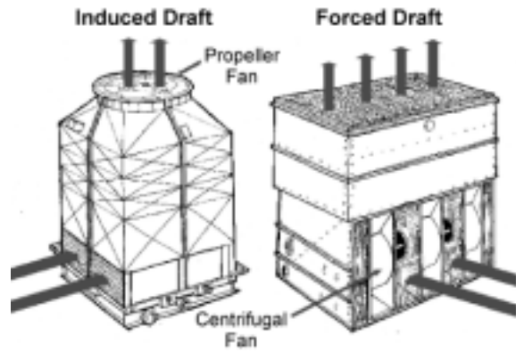
Cooling Towers
