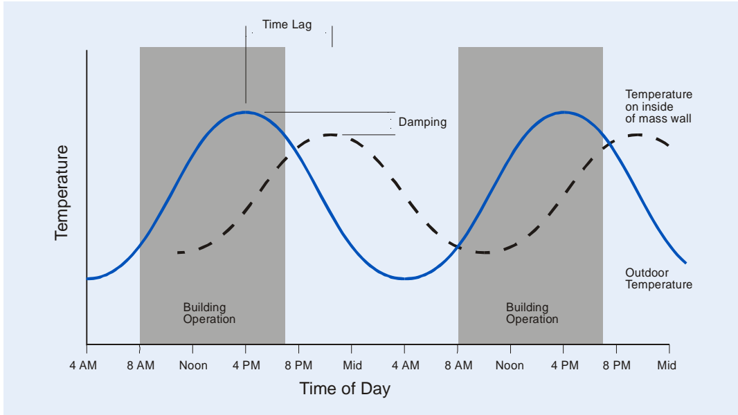
Figure 11 – Temperature Swing
