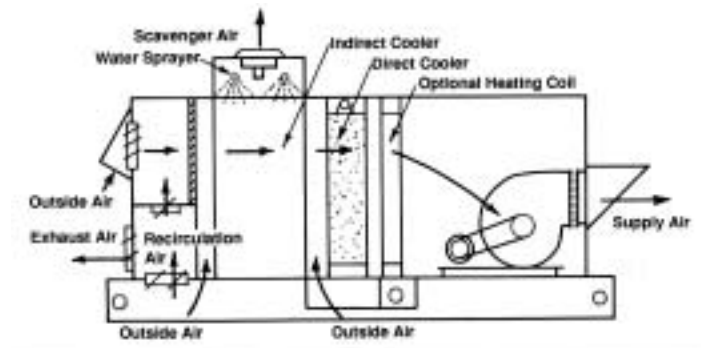
Evaporative Cooling System
