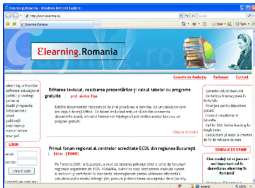
Figure 4. Elearning.Romania portal
