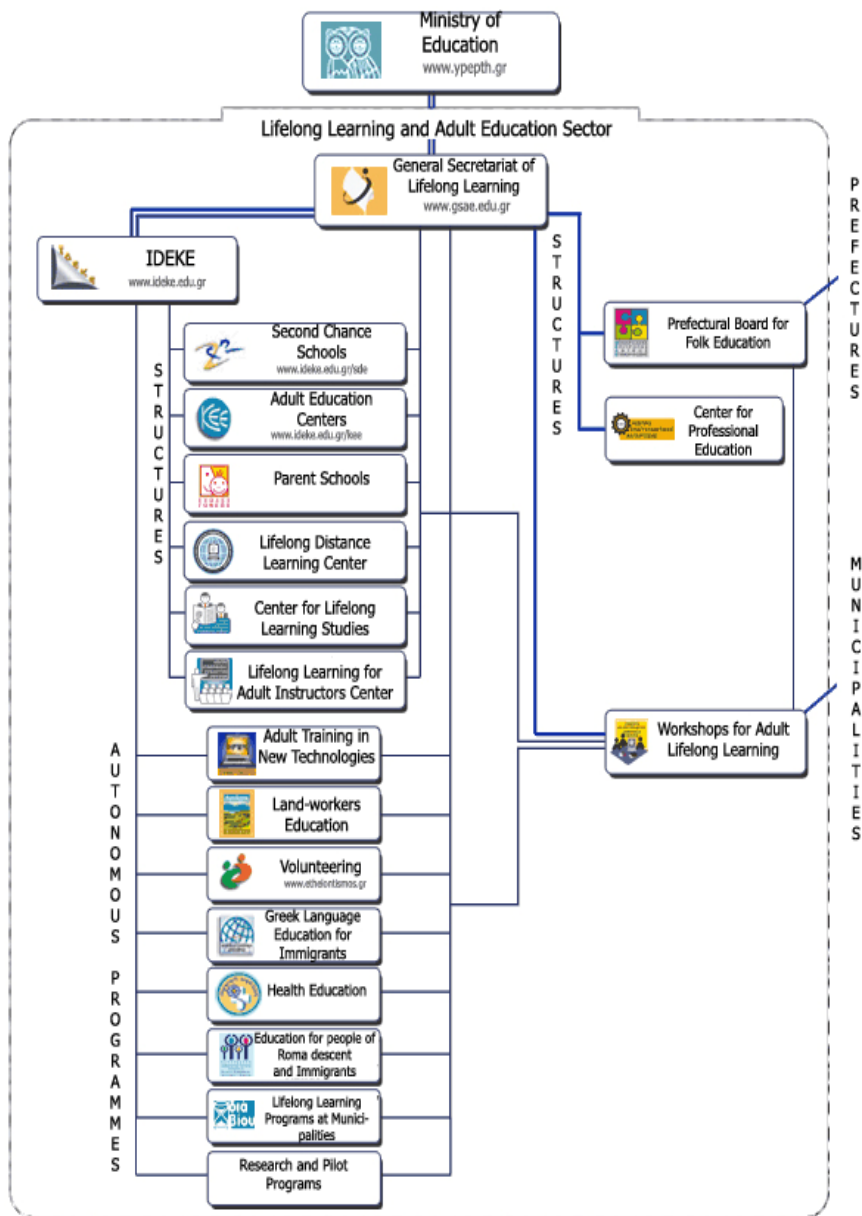
Figure 7. IDEKE Structure
