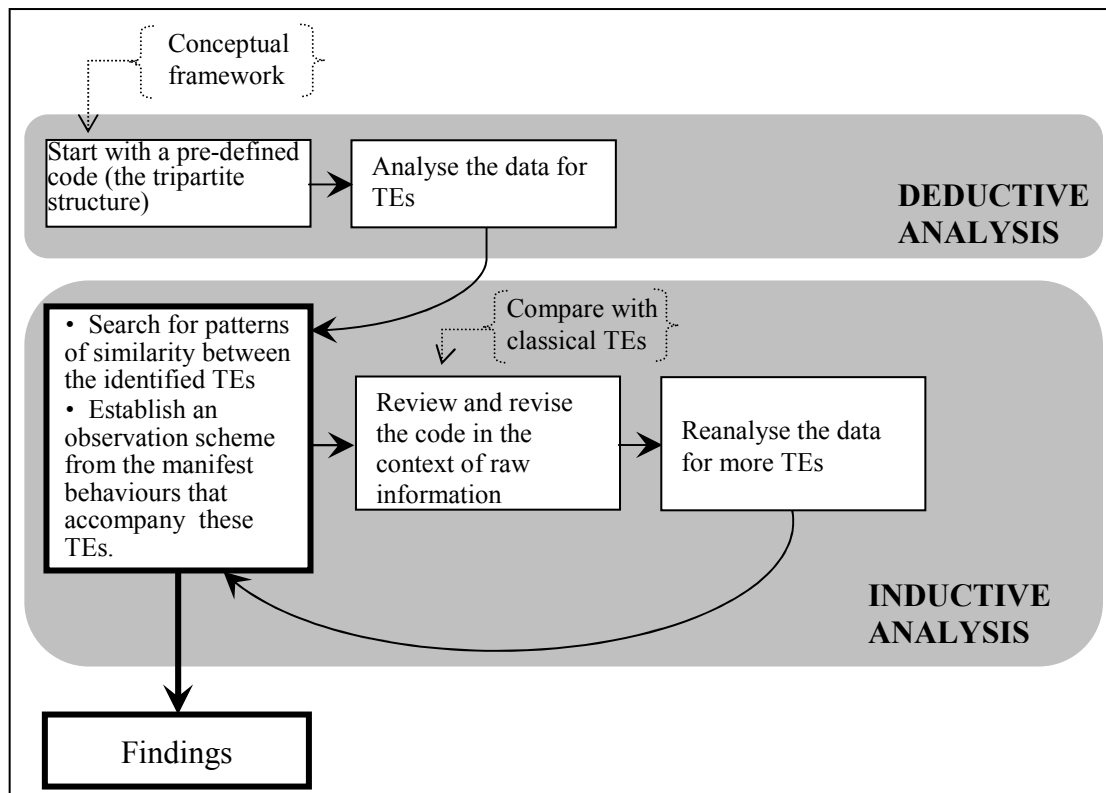
Figure 3.1: Analysis overview
