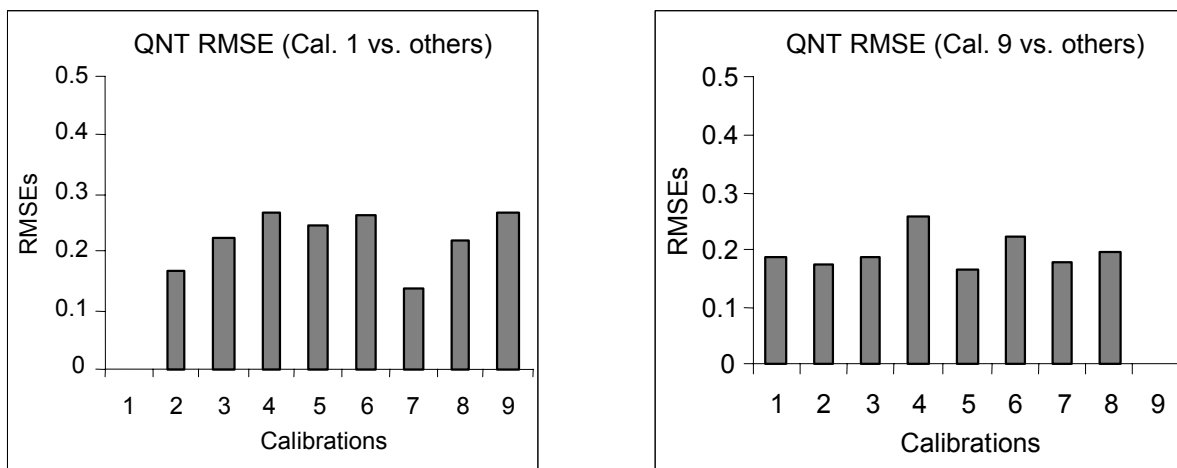
Figure 3. RMSEs between ability estimates on a response set scored by its own and other sets of item parameter estimates—Quantitative.
