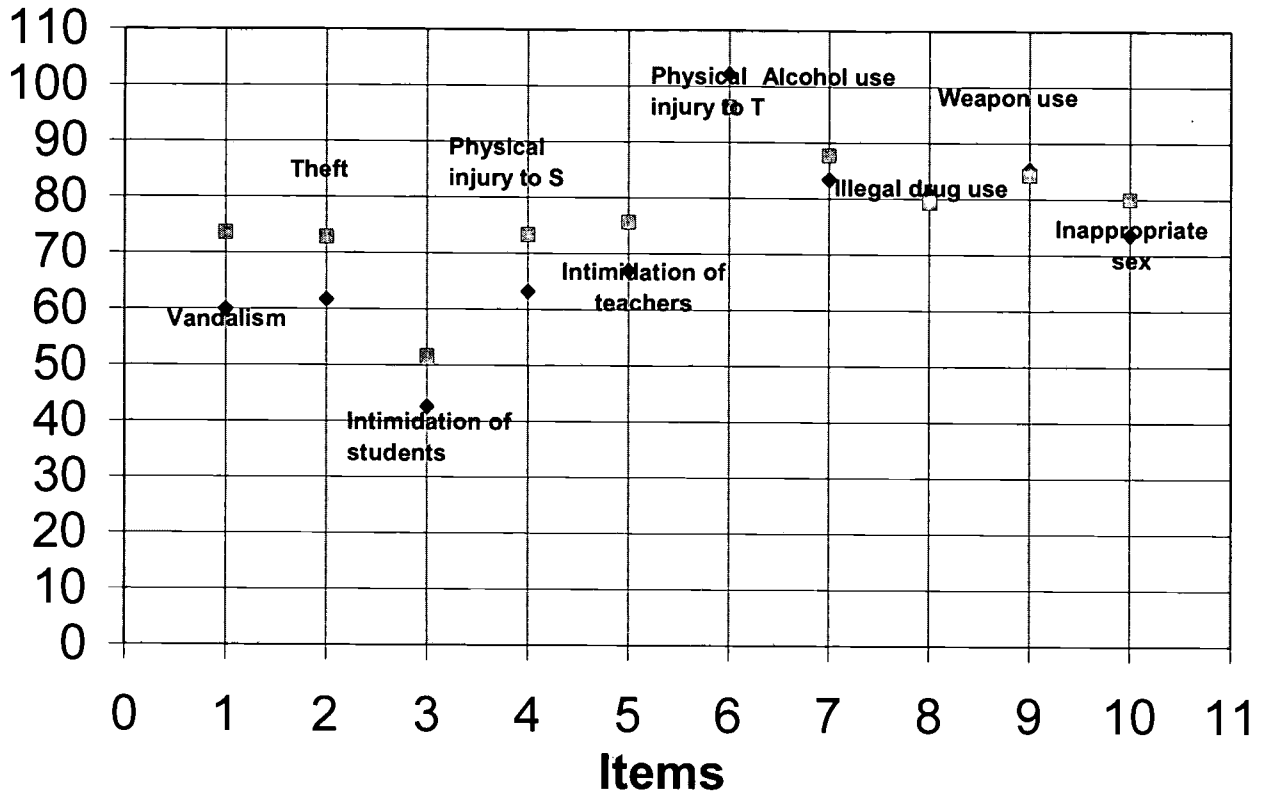
Figure 1. Comparisons of frequency and severity estimates Using TIMSS-R.
