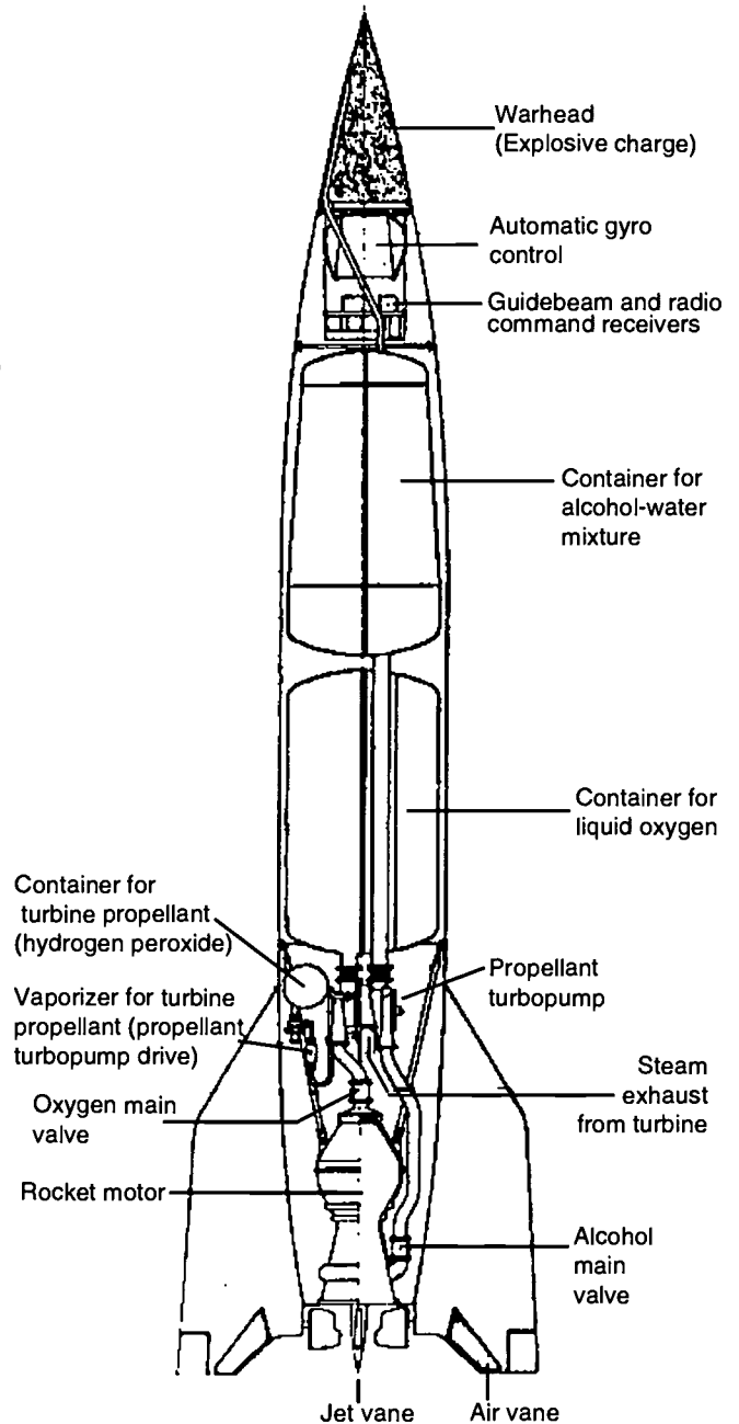
German V-2 (A-4) Missile
