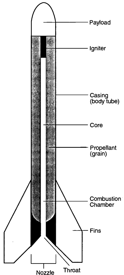
Solid Propellant Rocket
