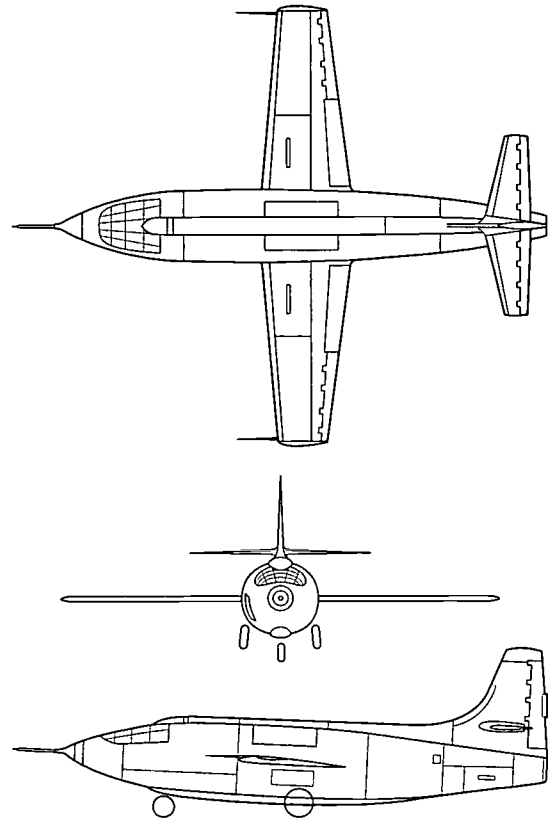
NACA X-1 Research Aircraft 1946
