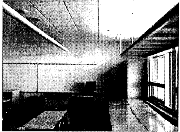
Classroom view shows how the outside light “bounces” into the room off the light shelves inside the room.
