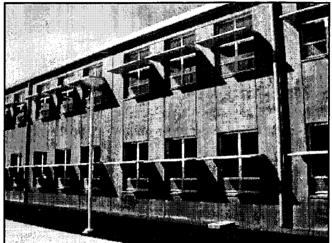
The new school walls are concrete and stained to look like basalt rock. Note the shading the light shelves provide to reduce glare and heat gain inside the classroom.
