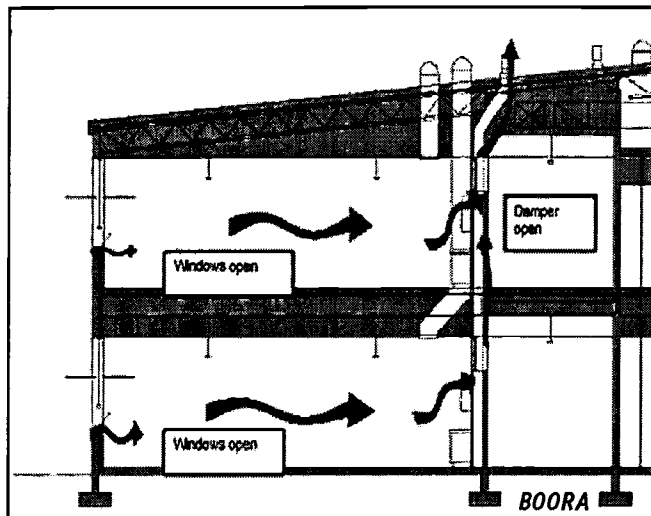
Green/red light system lets teachers know when to open windows.
