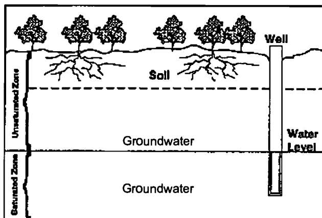
Diagram 1 Groundwater Zones
