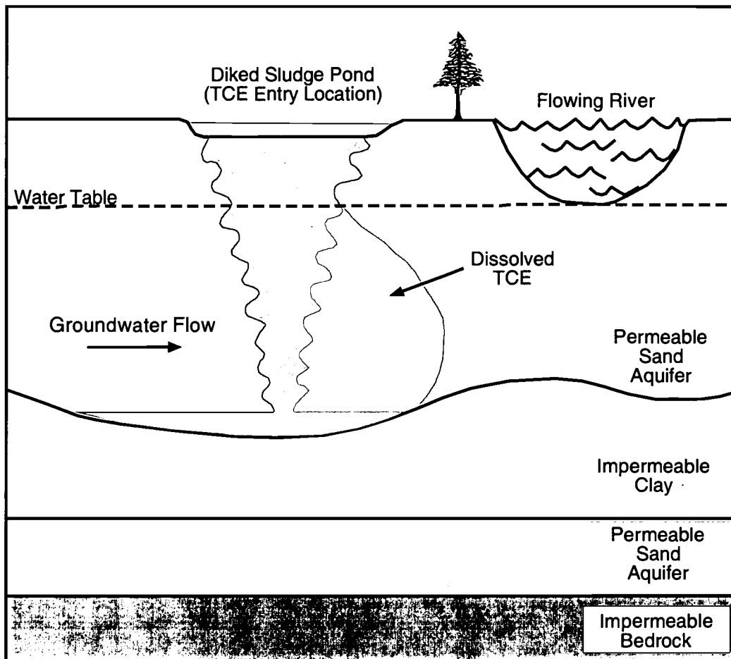
Map 3 Diked Sludge Pond, Cross-Section
