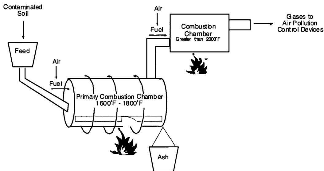
Diagram 2 Incineration Process
