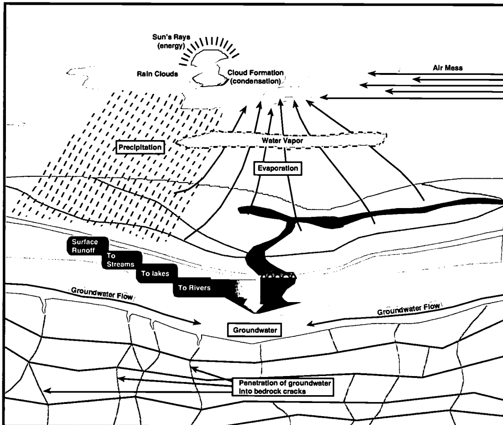
Diagram 2 Hydrologic Cycle
