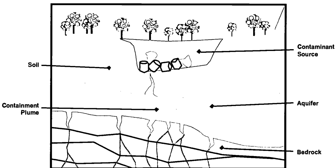
Diagram 3 Contaminated Groundwater
