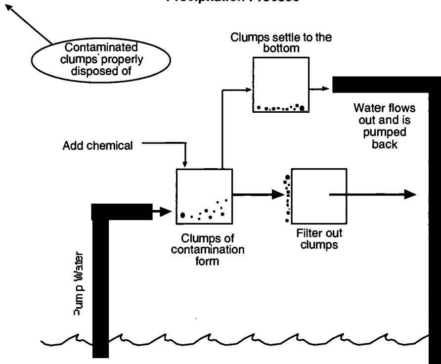
Diagram 1 Precipitation Process
