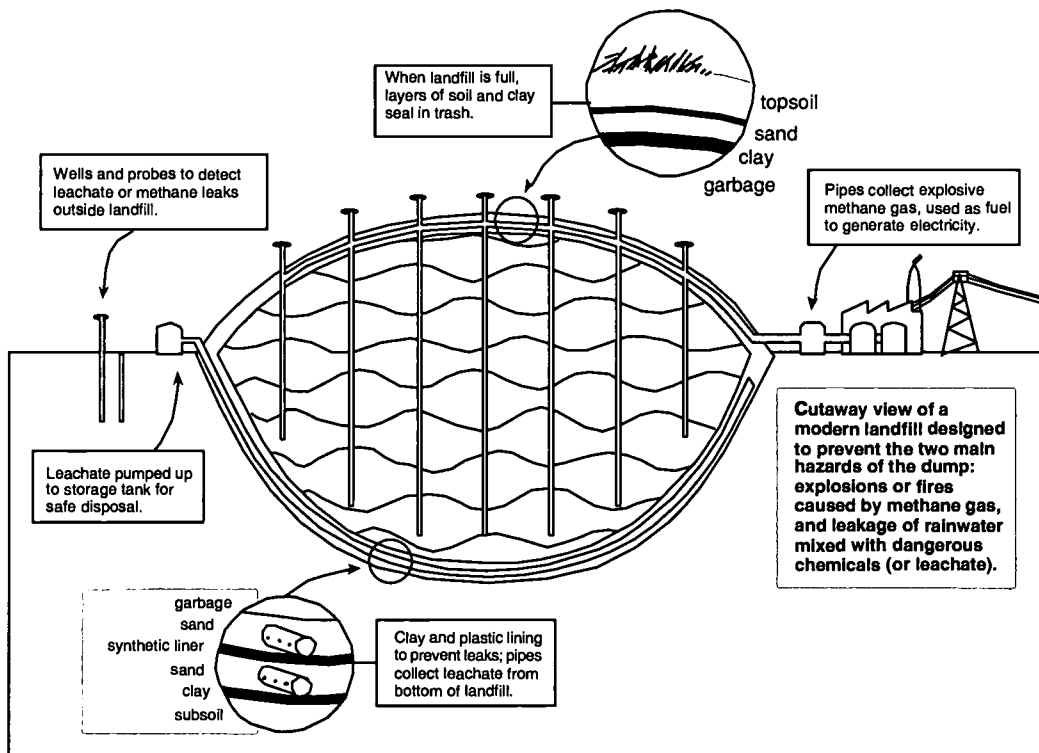
Diagram 1 Example of a Properly Closed Landfill
