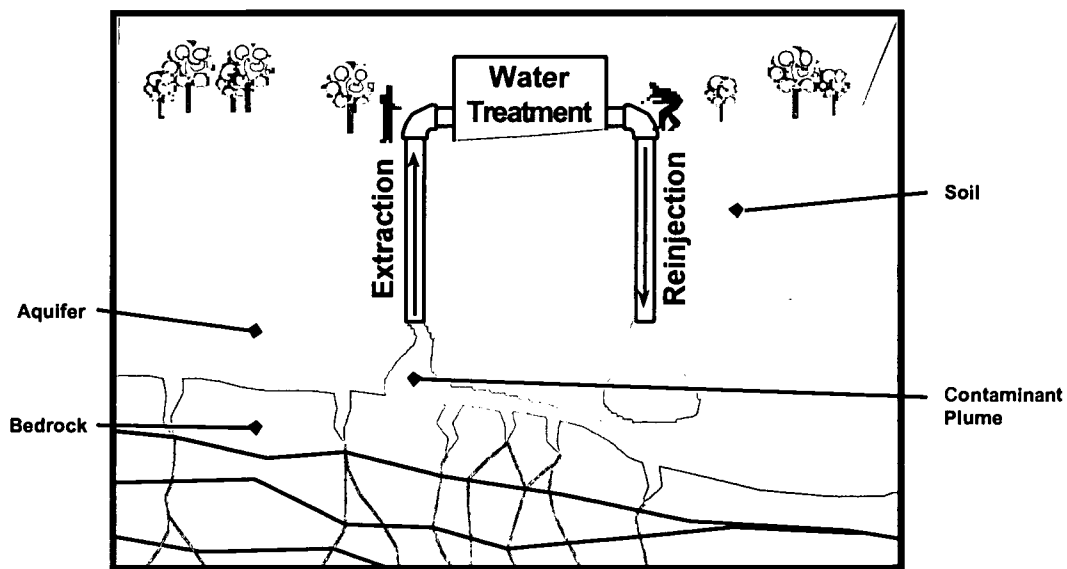
Diagram 4 Pumping and Treating Contaminated Groundwater
