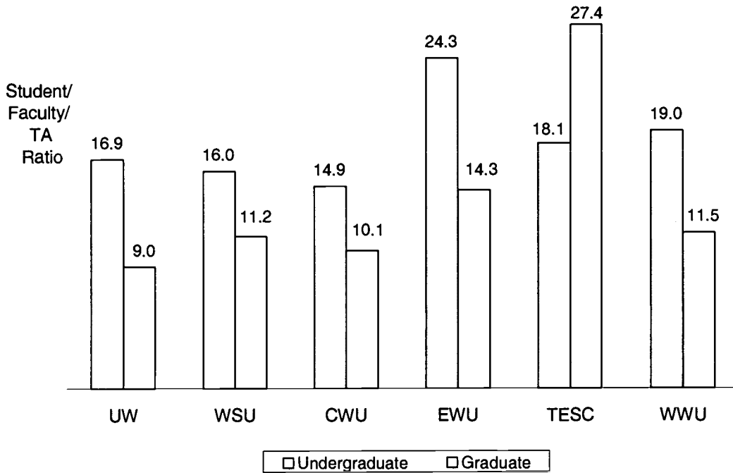
Graph 7: Student / Faculty & Teaching Assistant Ratios 2001-02 – Four-Year Institutions
