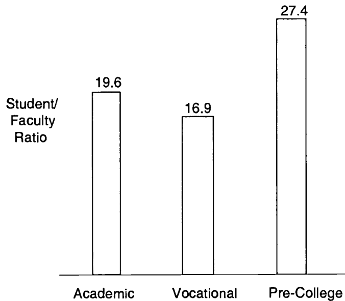
Graph 8: Student / Faculty Ratios 2001-02 – Two-Year Institutions
