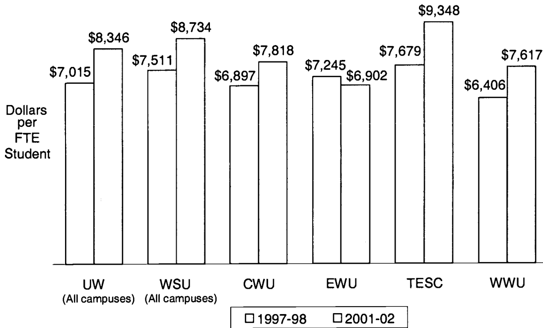
Graph 5: Cost of Instruction Comparison 1997-98 & 2001-02 Four-Year Institutions – Undergraduate
