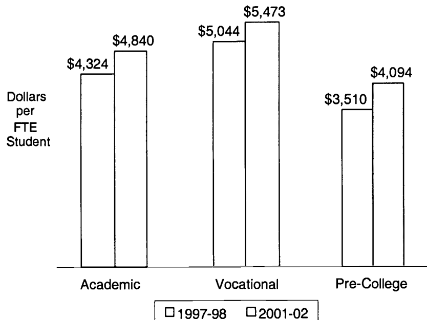
Graph 6: Cost of Instruction Comparison 1997-98 & 2001-02 Two-Year Institutions
