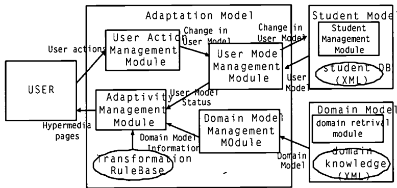
Figure 1: System architecture
