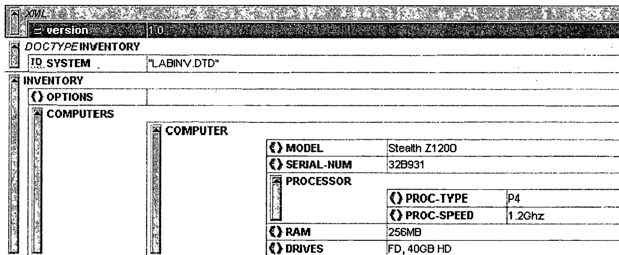
Fig. 7. XML Spy's Enhanced Grid View of the XML Document
