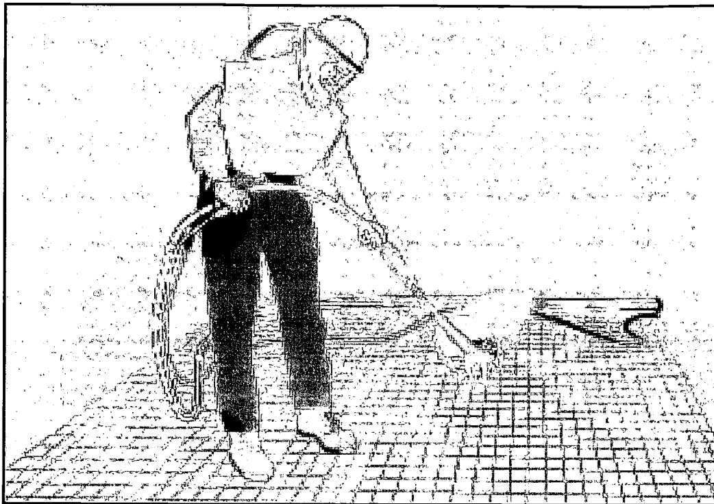
Figure 2. Sandblaster using proper respiratory protection inside a ventilated booth. Note that the worker is supplied with two separate air lines—one to supply fresh air for the worker to breathe and the other to supply air for sandblasting.
