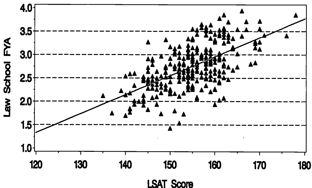
FIGURE 1. Best regression line for LSAT/FYA data, r = 0.62 .
