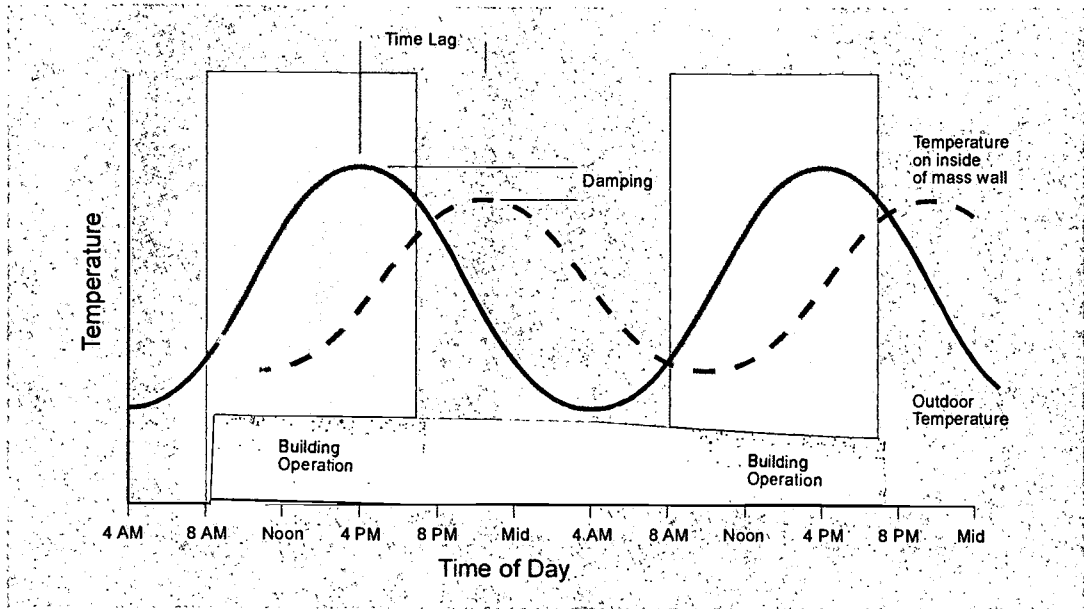
Figure 11 – Temperature Swing
