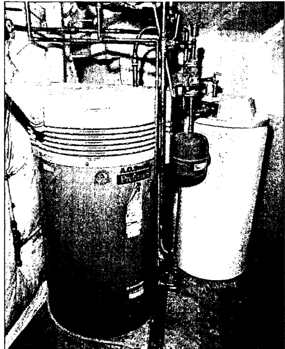
This central, high-efficiency boiler supplies hot water to two insulated storage tanks, providing hot water to six baths and a radiant floor heating system. NREL/PIX07925
