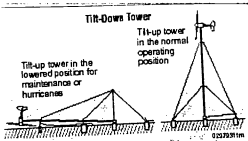
Figure 42 – Tilt-Down Towers
