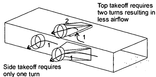
Figure 37 – Side Takeoff Vs. Top Takeoff
