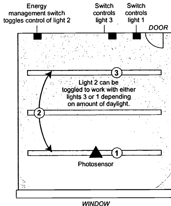
Figure 22 – Simple Windowed Classroom Control
