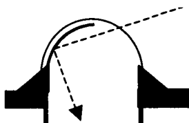
Figure 9 – Section of Reflective Half Dome NREL/PIX 11432
