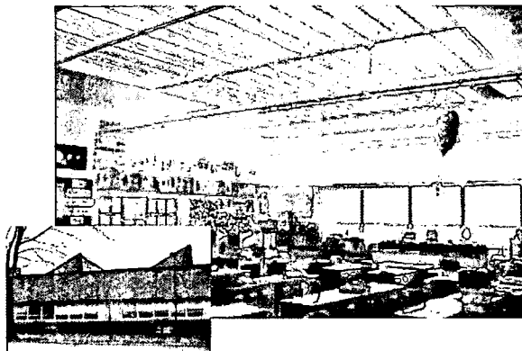
Central sawtooth monitor provides even illumination across desks in this classroom. NREL/PIX 11406
