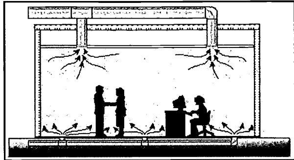
Displacement ventilation.
