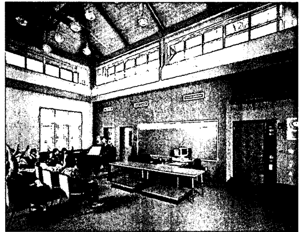
Clerestory windows provide a more uniform distribution of daylight across the space. NREL/PIX 11404
