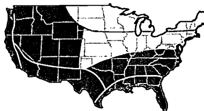
Radiant barriers are recommended for hot and coastal climates, over spaces cooled by air conditioners or natural ventilation. NREL/PIX 11331
