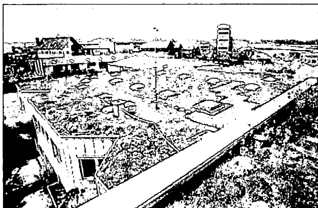
A vegetated roof reduces the amount of rainwater runoff while simultaneously minimizing heat build-up and providing insulation.
