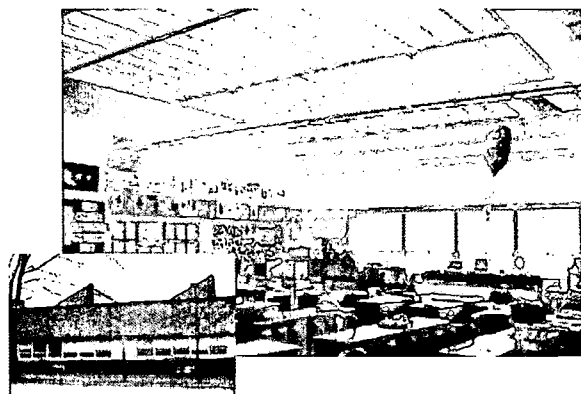
Guideline DL5: Central Toplighting from a sawtooth monitor with sun baffles is combined with DL1: View Windows to provide balanced illumination in a classroom. NREL/PIX 11406
