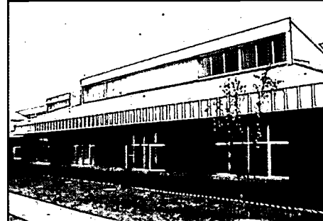
South-facing roof monitors and windows provide natural light in the classrooms.
