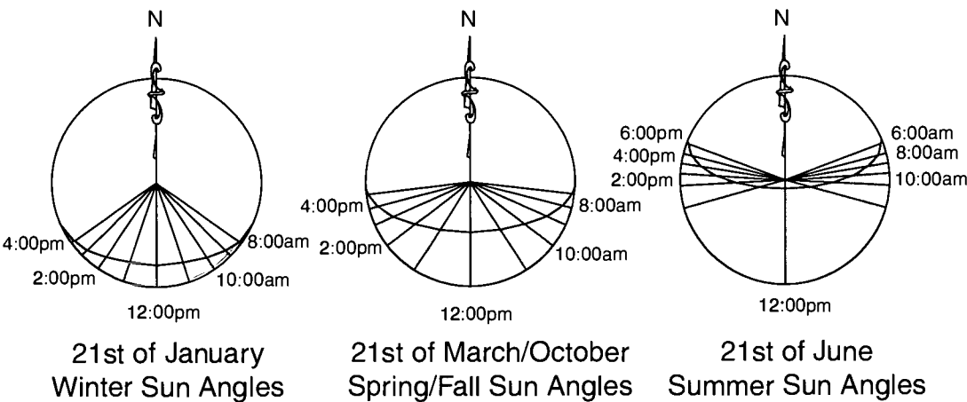
Sun Angles for Orlando, FL
