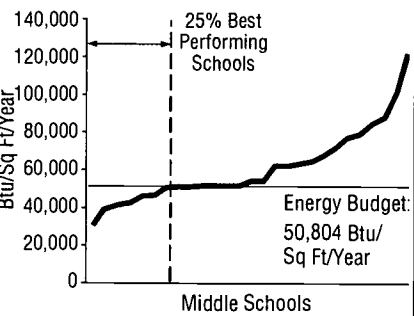
Orange County Middle Schools Annual Energy Consumption
