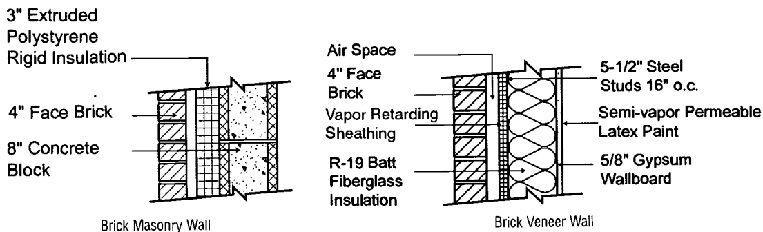
High-Mass Wall Sections
