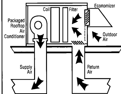
Economizer Cycle Diagram
