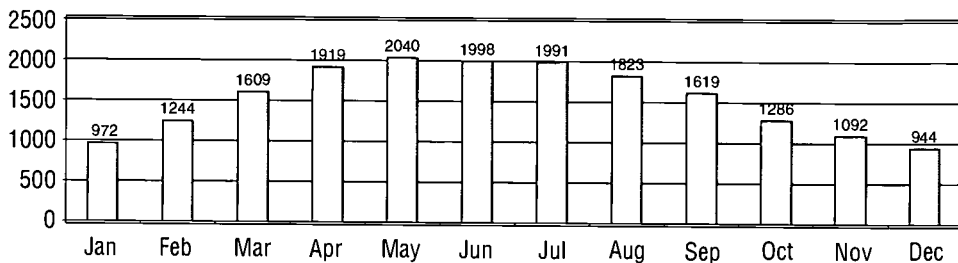
Average Incident Solar Radiation in Orlando (Btus/Square Foot/Day)
