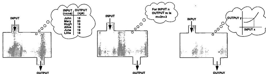
The function box as a table, a formula and a graph
