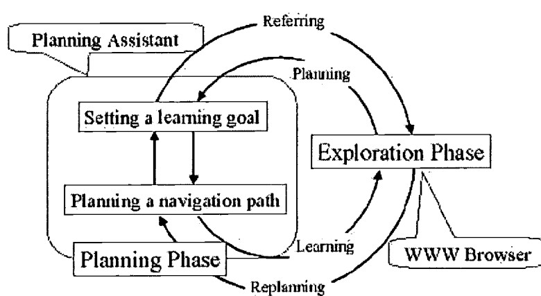
Figure 1: Learning process
