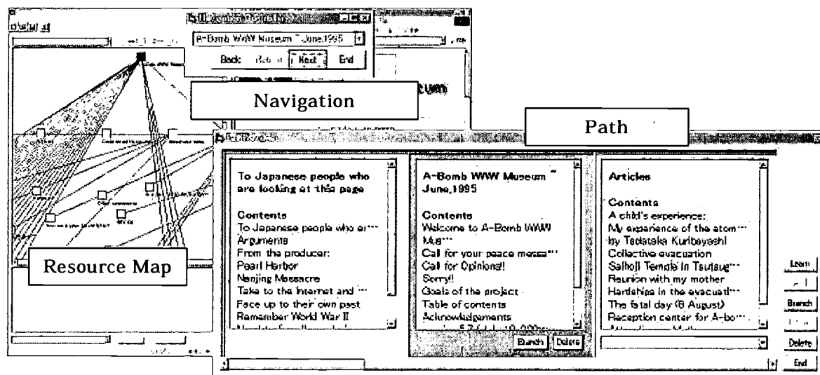
Figure 2: User Interface
