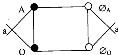
Bonding Configuration of a Open System of [AaO] Units
