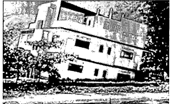
Figure 1. Excessive settlement in a building as a result of sand liquefaction. Earthquake of July 29, 1967, Caracas, Venezuela (National Geophysical Data Center)
