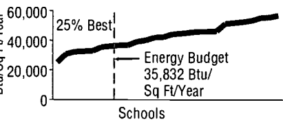
Paradise Valley Elementary Schools Annual Energy Consumption
