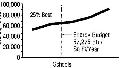
Paradise Valley Middle Schools Annual Energy Consumption
