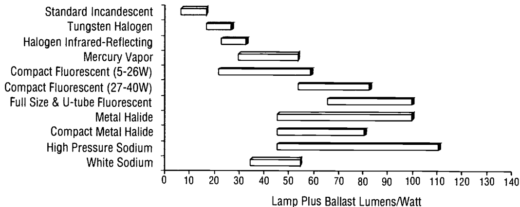
Comparison of Different Lamp Efficiencies
