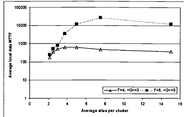
Figure 7: The impact of cluster size.
