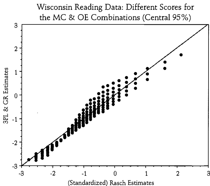
Figure 4.7. The values of EAP[\theta|x, x'] , computed using the 3PL/GR model combination, plotted against the values of MAP[\theta|x, x'] , computed using the Rasch model, using data from the Wisconsin third-grade reading test. (Only the points for the central 95% HDR of the score combinations are plotted)
