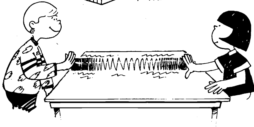
P-Wave
