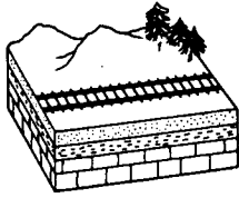
Pressure Direction
