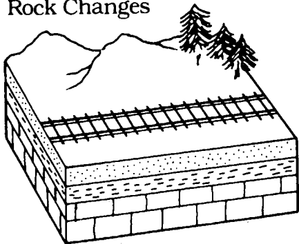
Rock Changes
