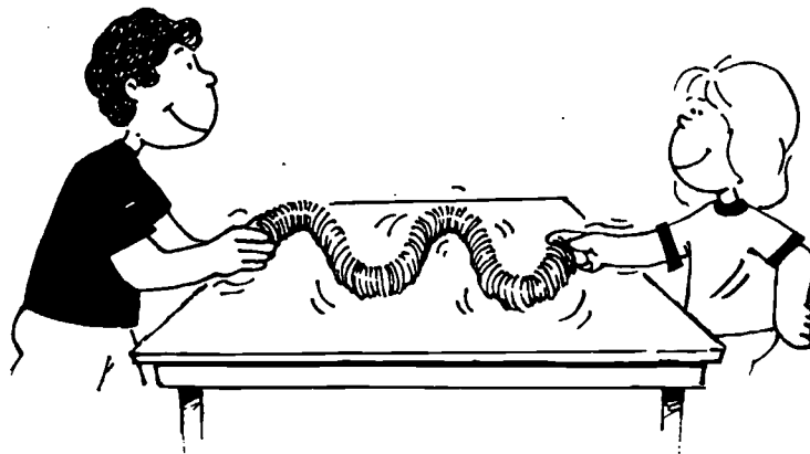
S-Wave
