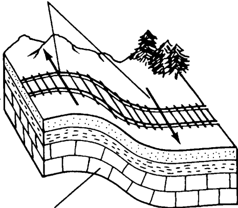
Deformed Rocks
