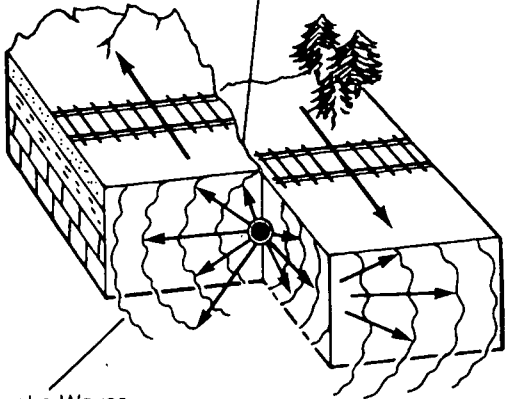
Earthquake Waves
