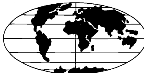
Earth land masses about 50,000,000 years into the future.
