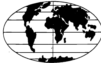
50,000,000 years from now
