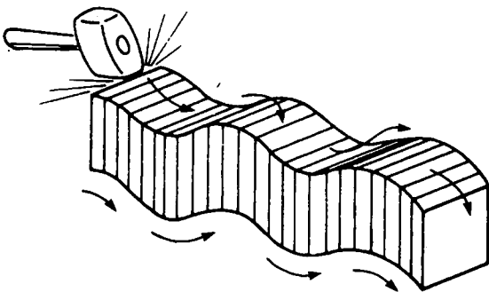
S-Wave
