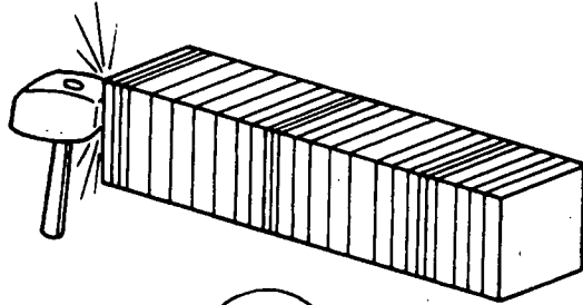
P-Wave
