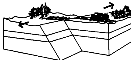
Horizontal Fault Movement
