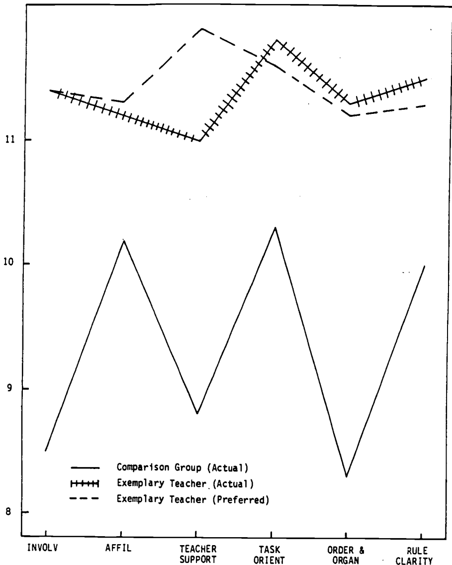
FIGURE 3. Profiles of Actual and Preferred Classroom Environment Scores for an Exemplary Biology Teacher and Actual Environment Scores for a Comparison Group
