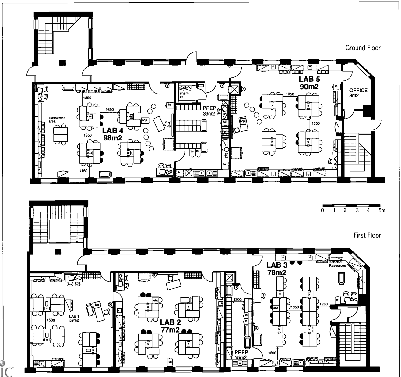
Figure 6/4 Case Study 1, Option C
