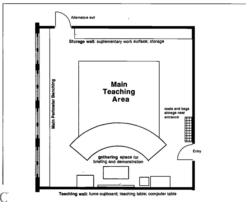
Figure 2/5 Zoning Diagram
