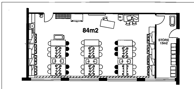
Figure 6/8 Case Study 2, Option C
