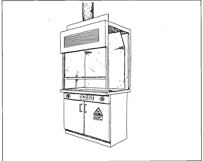
Figure 4/8 Fixed Fume Cupboard with vented corrosives cabinet underneath
