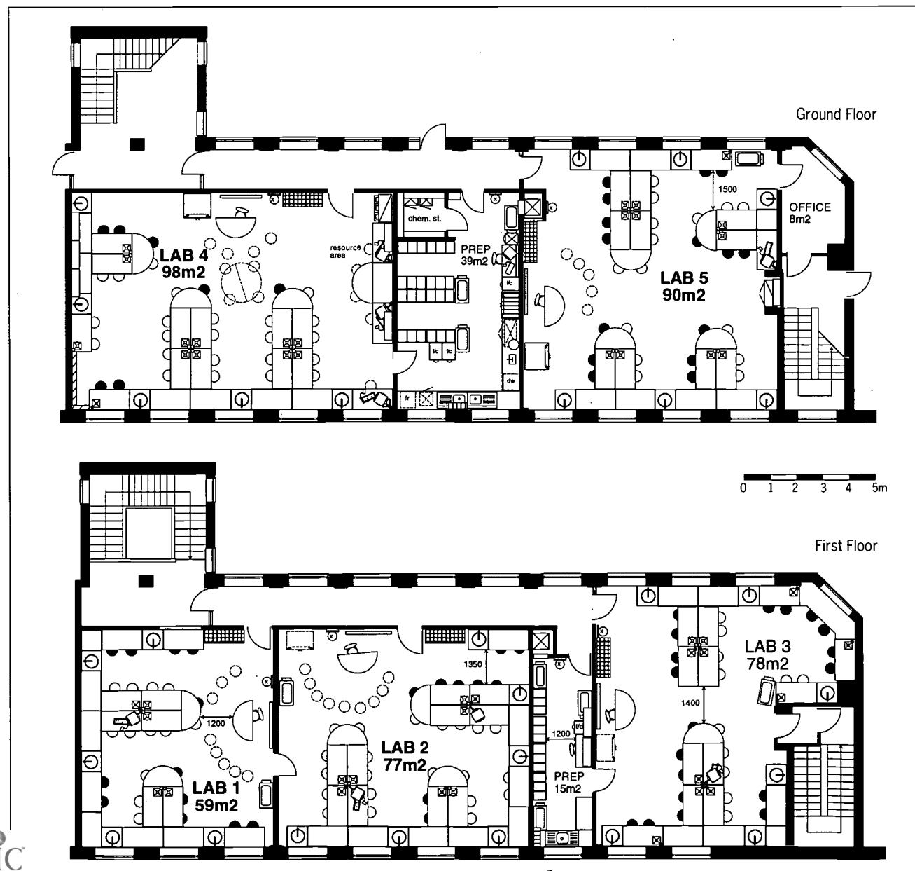
Figure 6/3 Case Study 1, Option B
