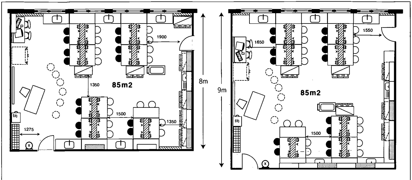
Spine & Perimeter Sink (Figure 2/12)
