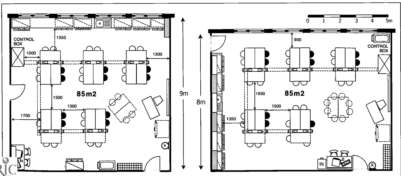
Figure 2/11 Labkit Workstation
