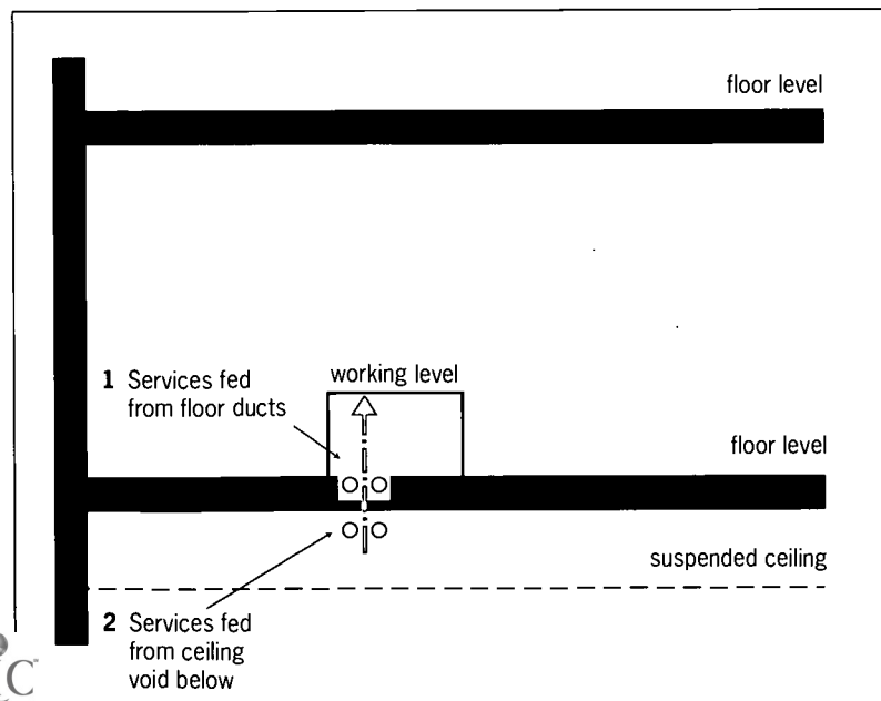
Figure 2/8 Underfloor Servicing
