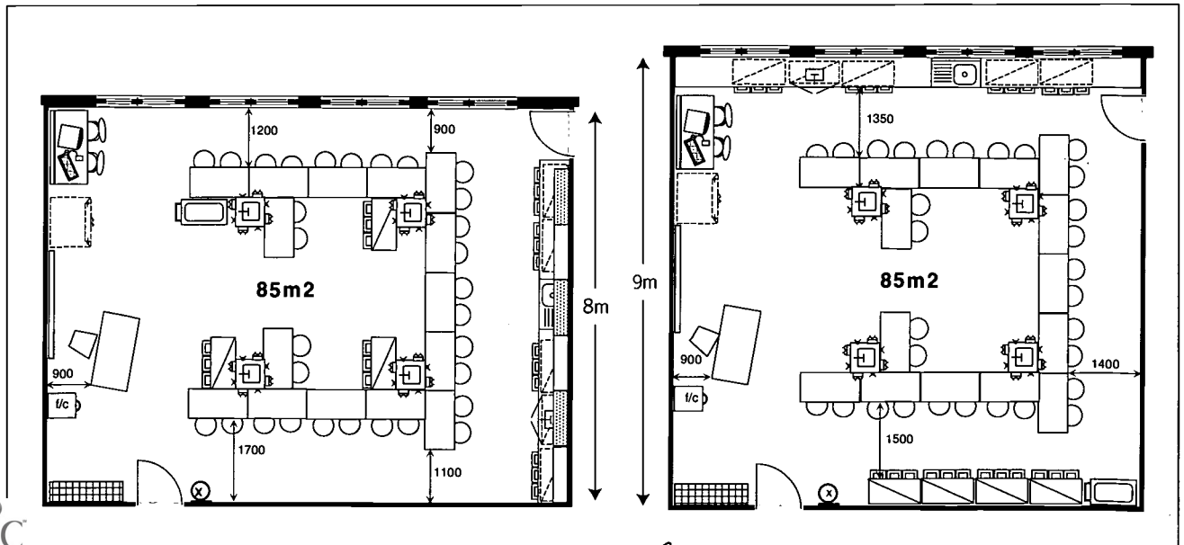
Figure 2/17 8 Person Bollard Option B
