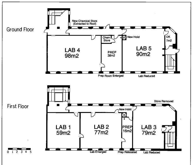
Figure 1/9 Floor Plans as Adapted
