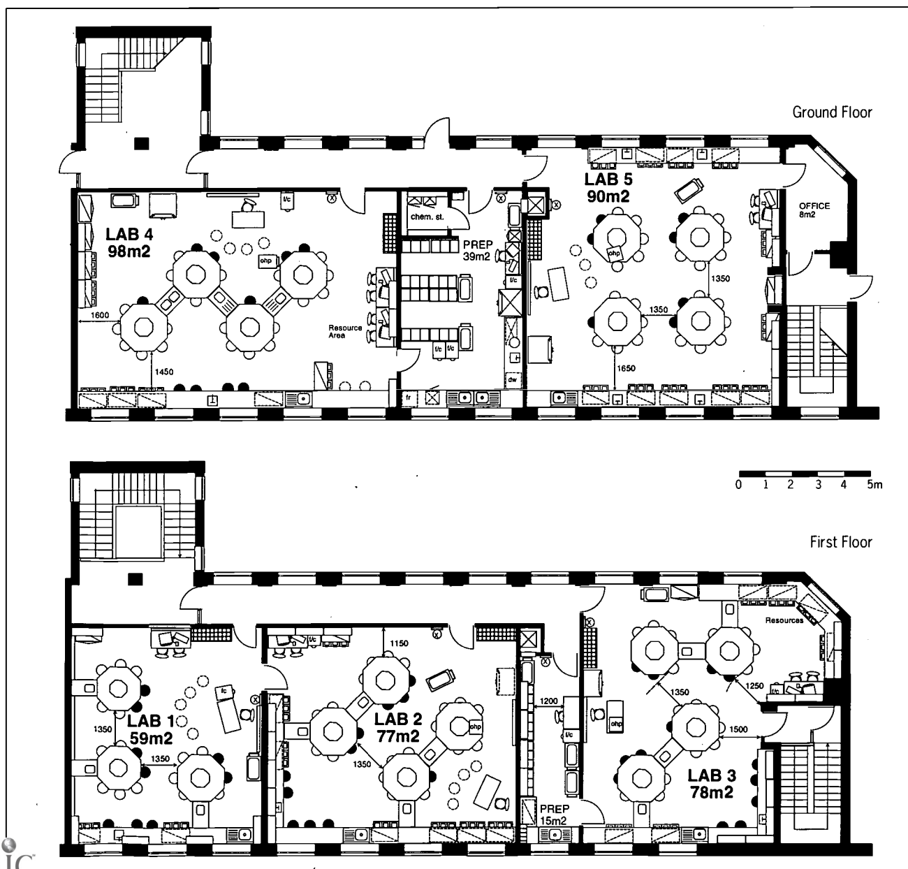
Figure 6/2 Case Study 1, Option A
