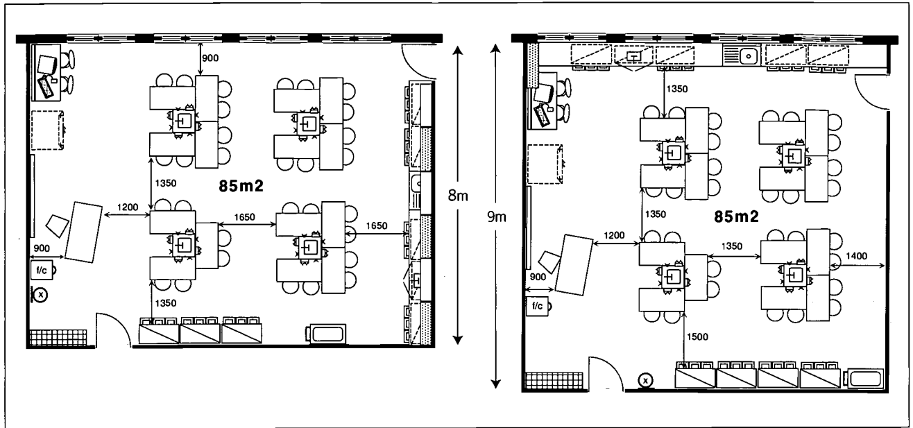
Figure 2/16 8 Person Bollard Option A
