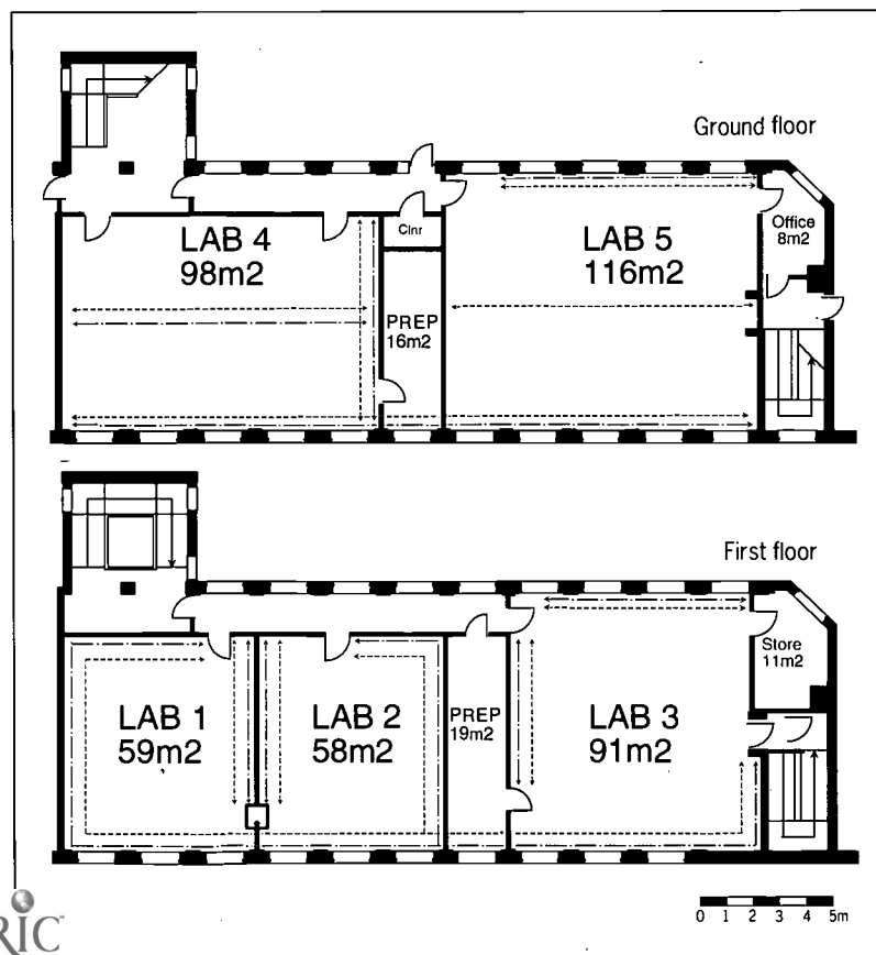
Figure 6/1 Case Study 1, Servicing arrangement of existing building
