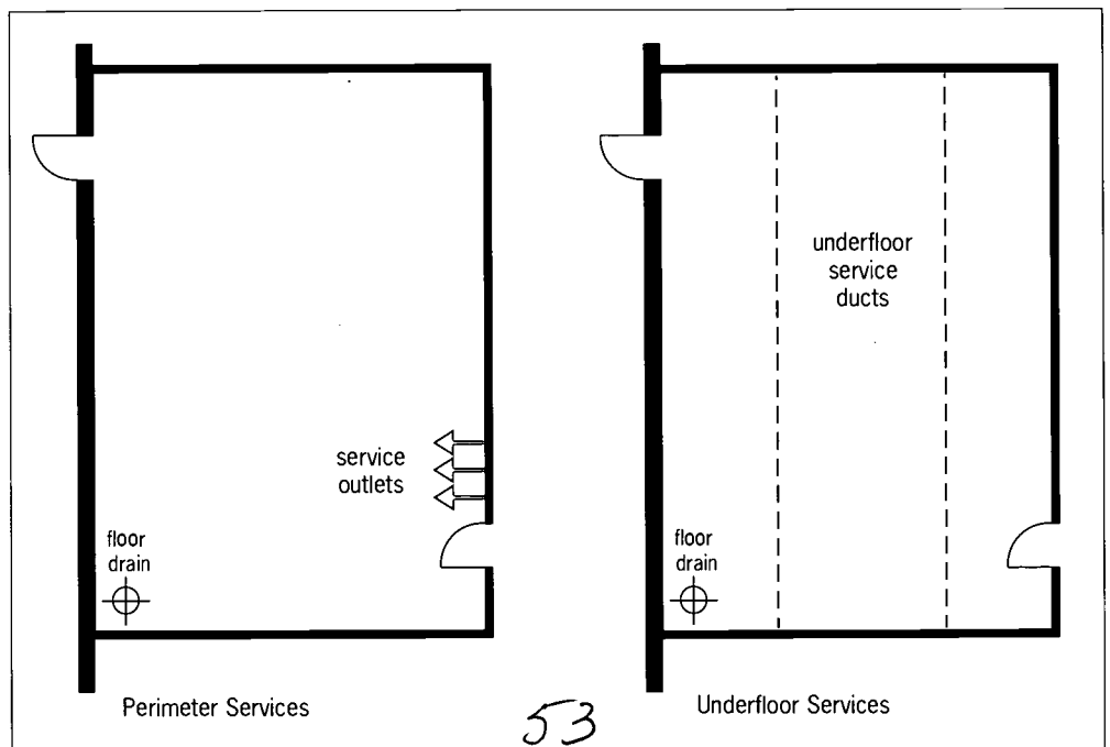
Figure 7/1 Laboratory Plans Used for Comparative Cost Study
