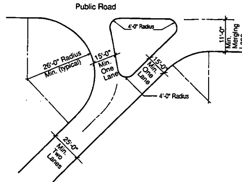
TYPICAL "Y-INTERSECTION" FOR BUSES
