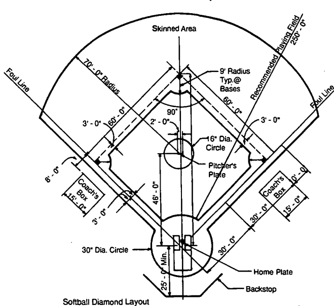
Softball Diamond Layout
