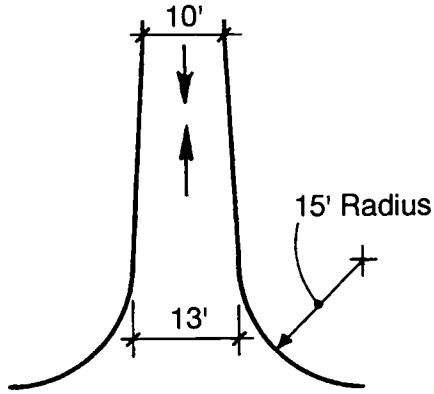
One Way Single Lane Entrance - Exit
