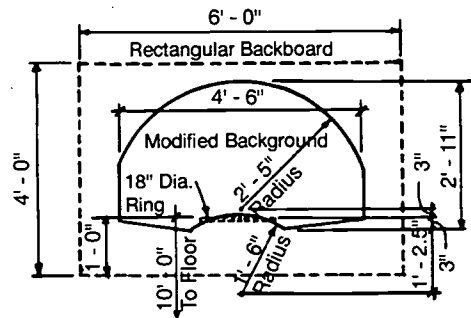
Backboard Detail
