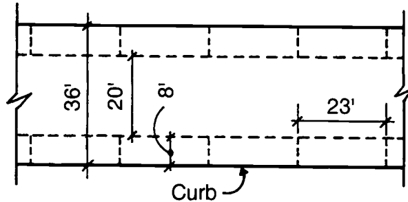
Typical Two Lane Drive Parallel Parking Each Side
