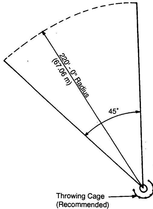
SECTOR LAYOUT - DISCUS THROW
