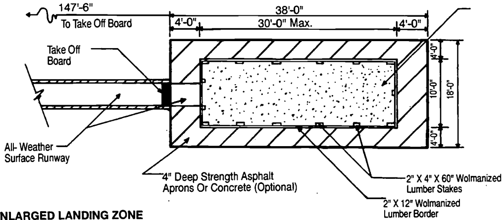
ENLARGED LANDING ZONE
