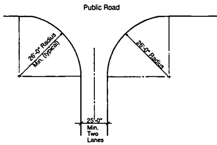
TYPICAL "T-INTERSECTION" FOR BUSES
