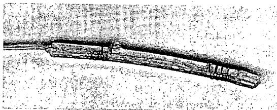
Figure 1. The IM electrode used in these studies consisted of a silicone tube. Two wires were passed through and wrapped around the tube to act as the anode and cathode.
