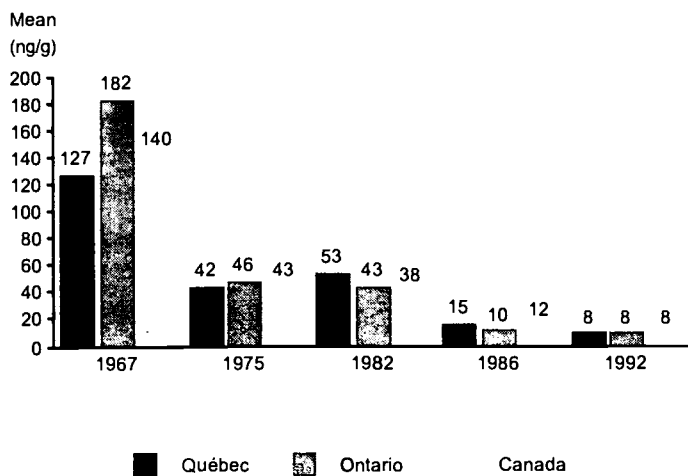
Trends in Levels of DDT in Human Breast Milk Québec, Ontario, Canada, 1967-1992
