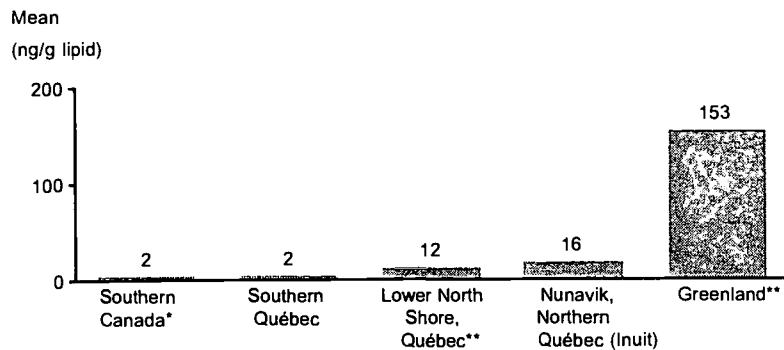
Concentrations of Mirex in Human Milk Fat 1989-1990
