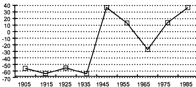
Trends in Canadian and Global Average Air Temperatures 1905-1985
