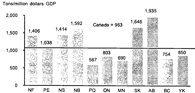
Carbon Dioxide Emissions in Relation to Provincial Economies Canada, Provinces and Territories, 1990
