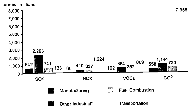
Emissions of Air Pollutants, by Sector, Canada, 1990
